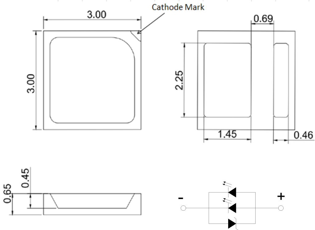
Figure 10: Drawing for SMD 3030
