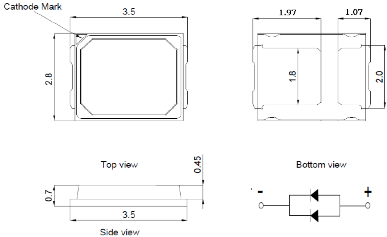
Figure 11: Drawing for SMD 2835
