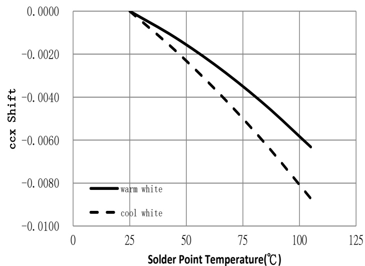
Figure 5: Typical ccx Shift vs. Solder Point Temperature
