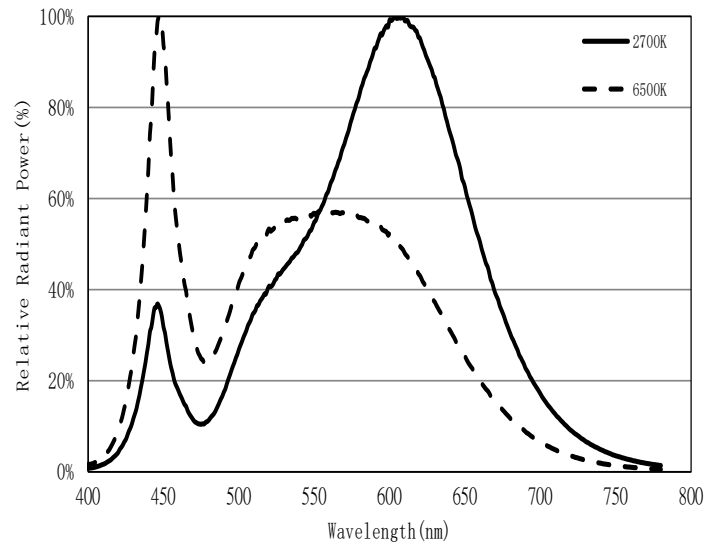
Figure 9: Typical Color Spectrum
