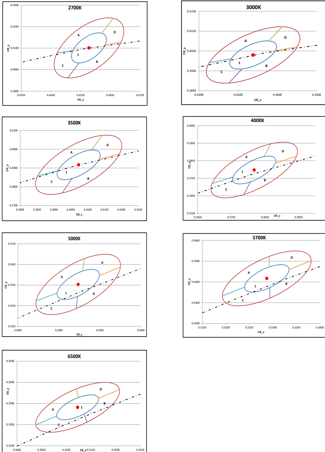
Figure 1: C.I.E. 1931 Chromaticity Diagram ( hot-color targeted at T_{sp}=85^{\circ}\text{C} )
