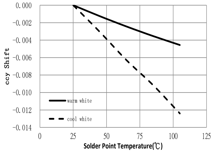
Figure 6: Typical ccy Shift vs.Solder Point Temperature
