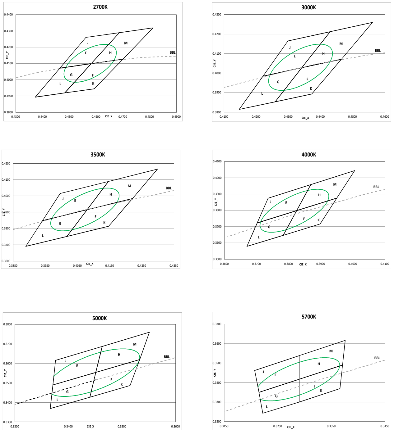
Figure 1: C.I.E. 1931 Chromaticity Diagram (8 Color Bin Structure, Targeted at T_{sp}=25^{\circ}\text{C} )
