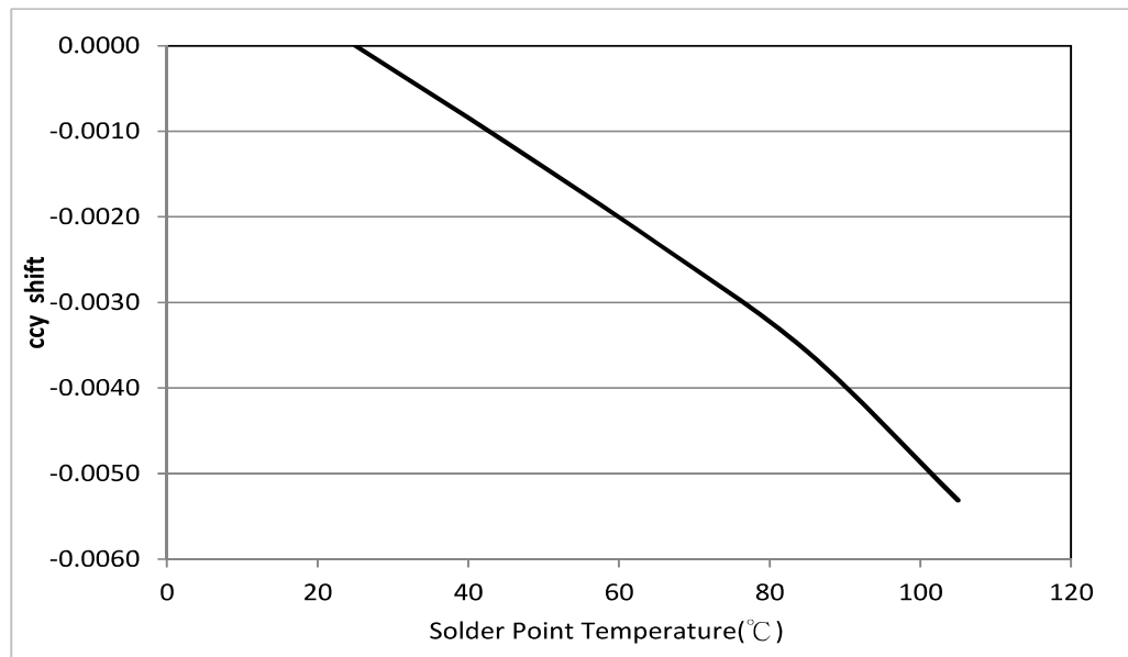
Figure 6: Typical ccy Shift vs. Solder Point Temperature
