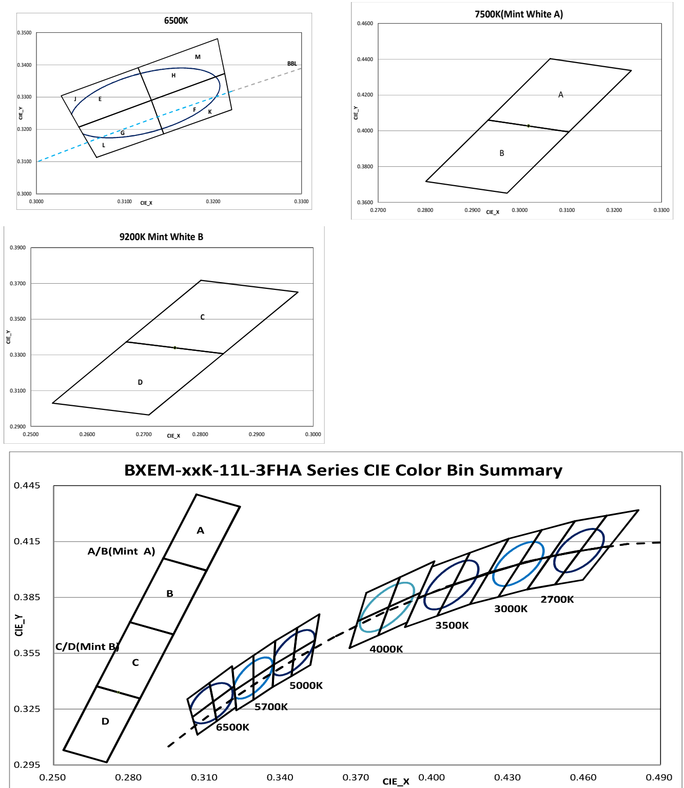
Figure 1: C.I.E. 1931 Chromaticity Diagram (8 or 2 Color Bin Structure, Targeted at T_{sp} = 25^{\circ}\text{C} )
