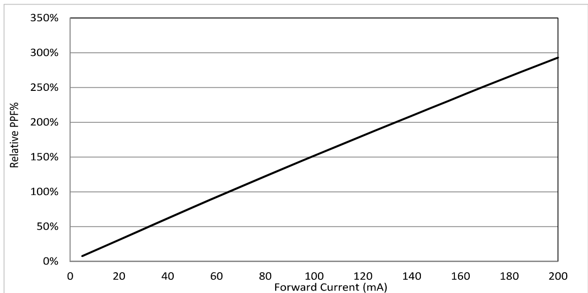
Figure 3: Relative Luminous PPF vs. Forward Current ( T_{sp}=25^{\circ}\text{C} )
