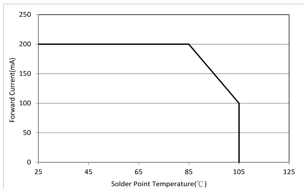
Figure 7: Drive Current vs Solder Point Temperature
