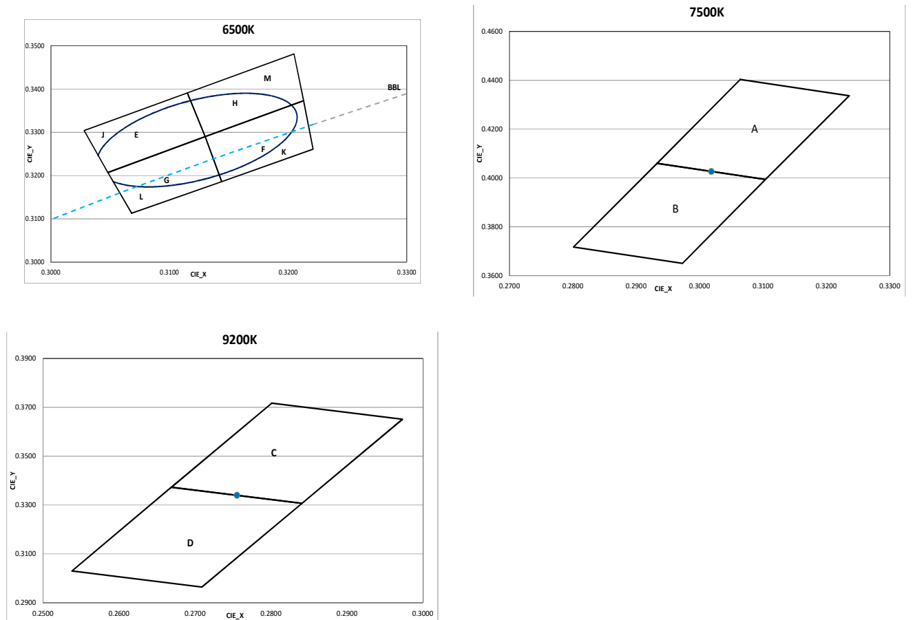
Figure 1: C.I.E. 1931 Chromaticity Diagram (5 Color Bin Structure, Hot-color Targeted at T_{sp}=85^{\circ}\text{C} )
