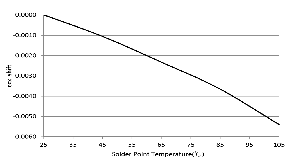
Figure 5: Typical ccx Shift vs. Solder Point Temperature
