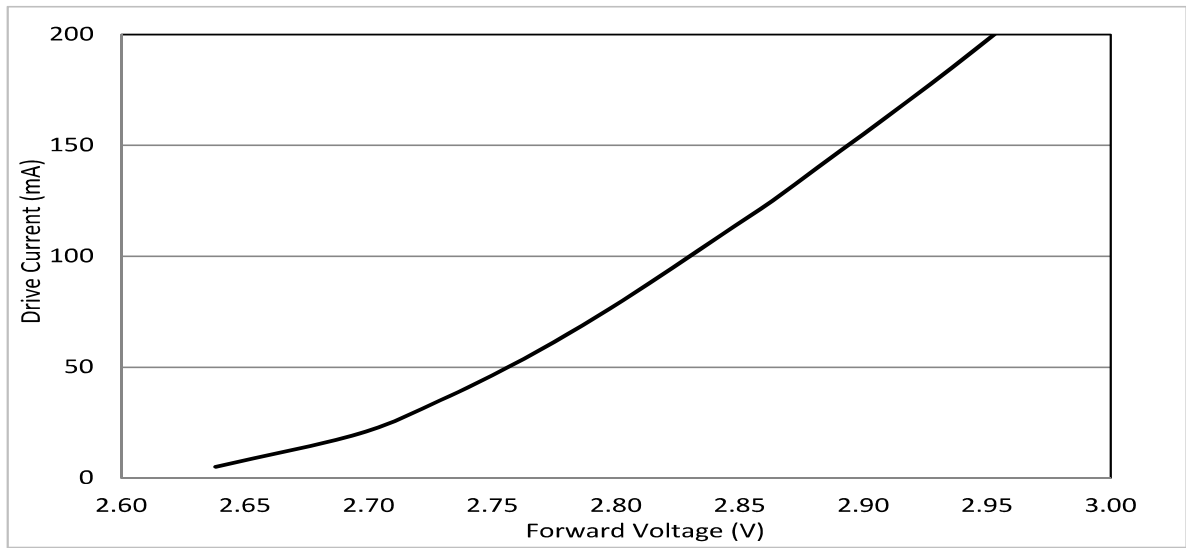
Figure 2: Drive Current vs. Forward Voltage ( T_{sp}=25^{\circ}\text{C} )
