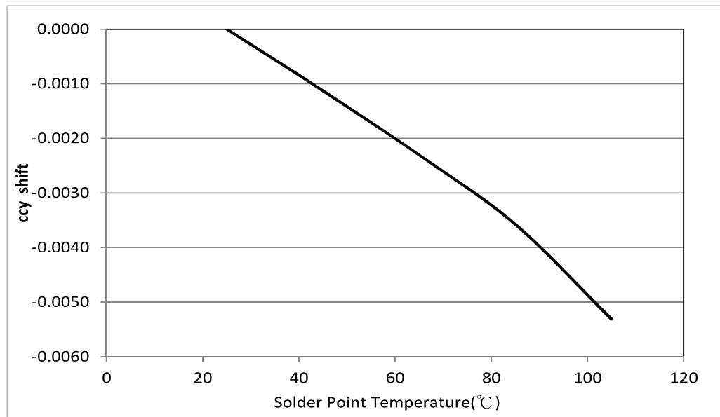
Figure 6: Typical ccy Shift vs. Solder Point Temperature
