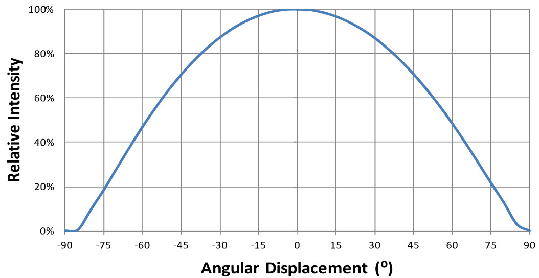
Figure 8: Typical Spatial Radiation Pattern at 65mA, T_{sp}=25^{\circ}\text{C}
