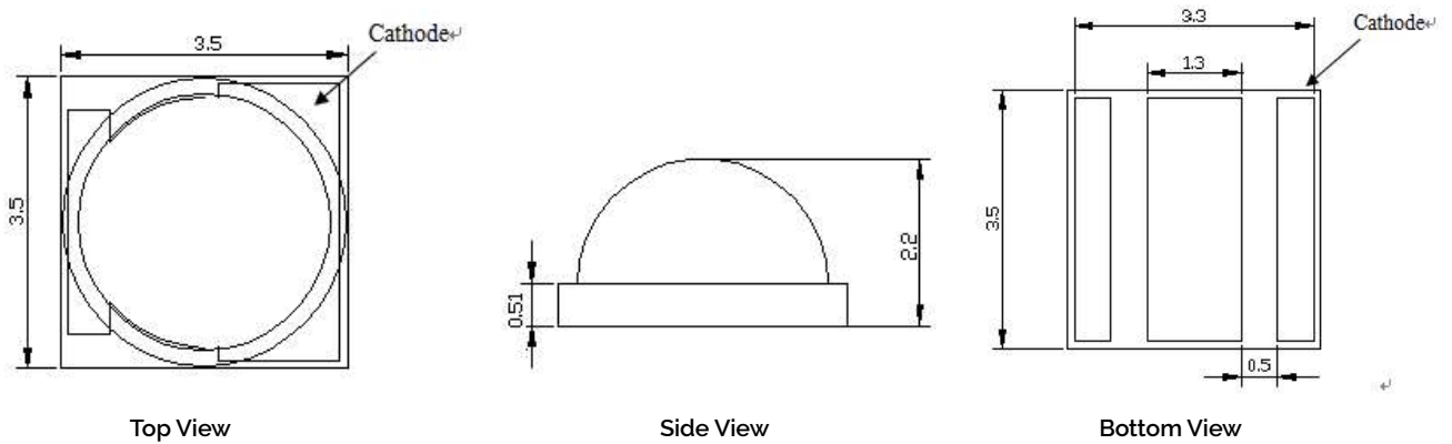
Figure 8: Drawing for SMD 3535
