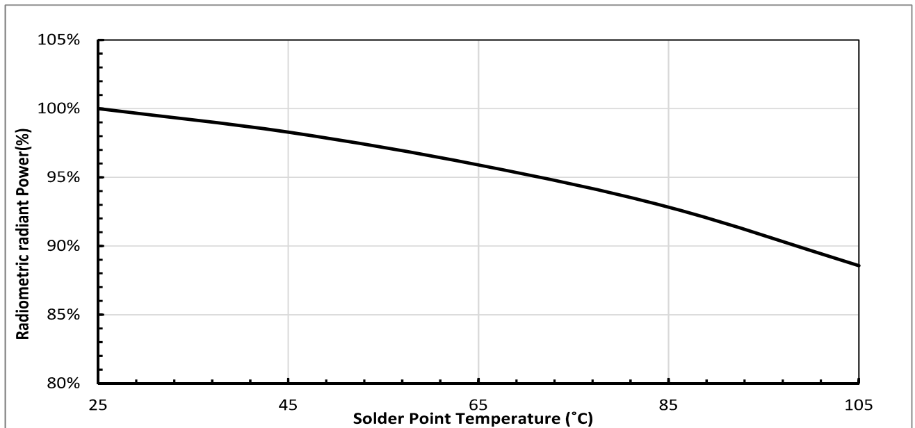
Figure 3: Relative Total Radiant Radiometric vs. Solder Point Temperature
