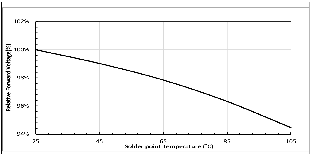
Figure 4: Relative Forward Voltage vs. Solder Point Temperature
