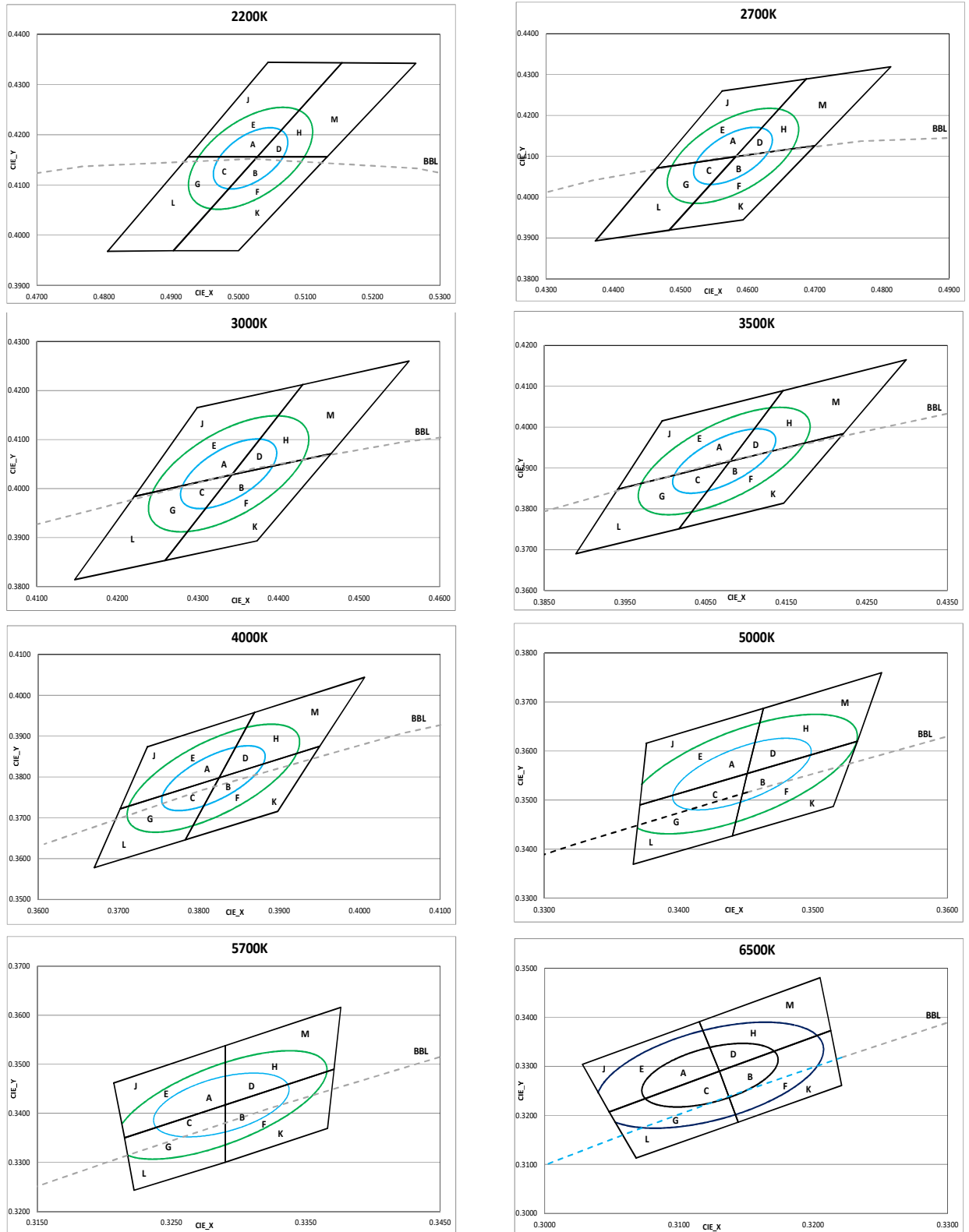
Figure 1: C.I.E. 1931 Chromaticity Diagram (12 Color Bin Structure, Color Targeted at T_{sp} = 25^{\circ}\text{C} )
