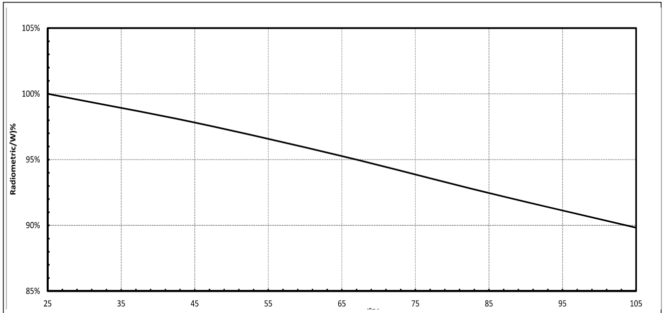
Figure 3: Typical Relative Total Radiant Radiometric vs. Solder Point Temperature
