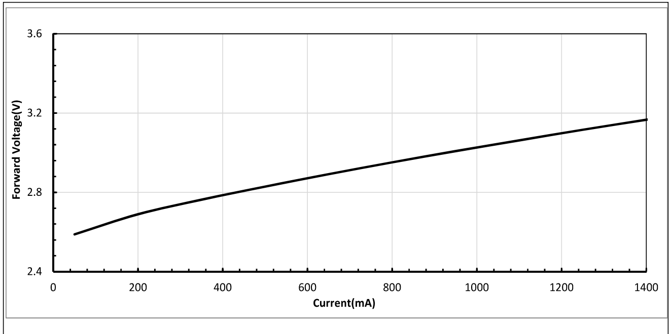
Figure 1: Drive Current vs. Voltage ( T_{sp}=25^{\circ}\text{C} )
