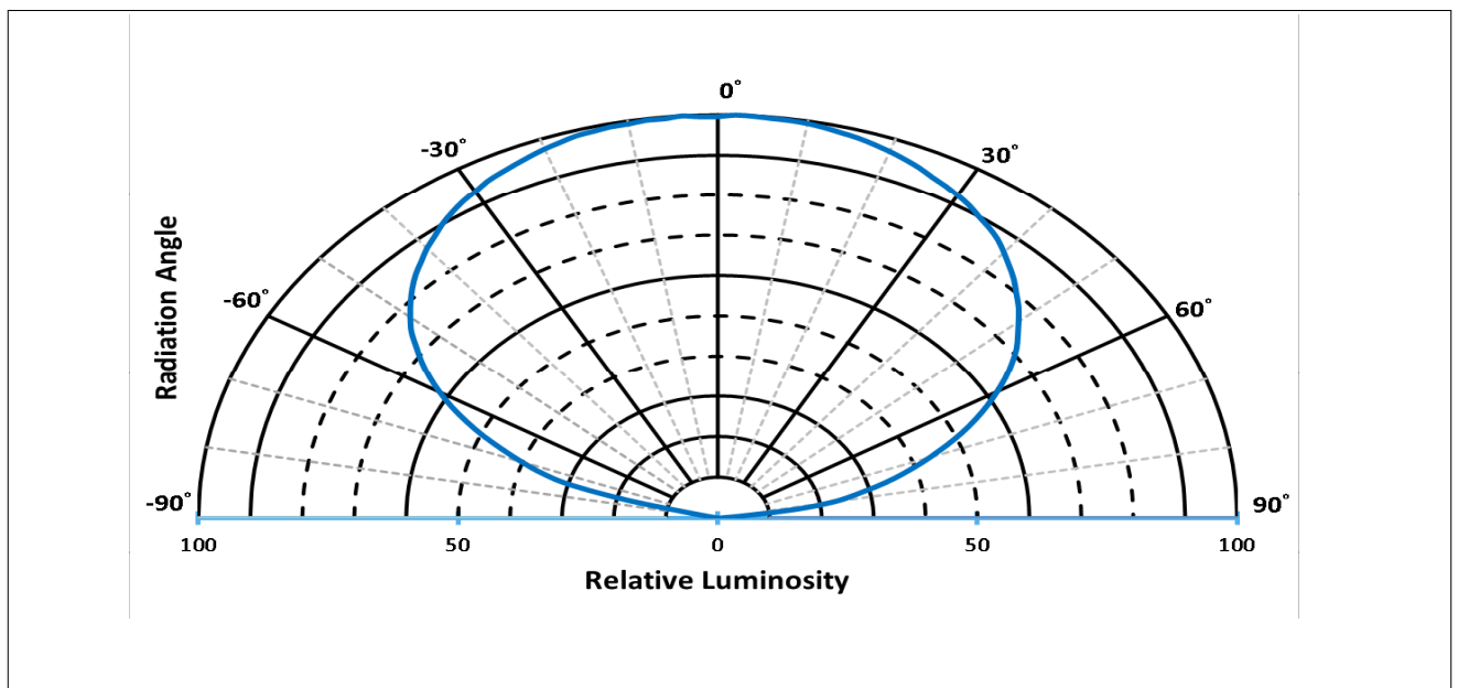
Figure 6: Typical Polar Radiation Pattern at 700mA, T_{sp}=25^{\circ}\text{C}
