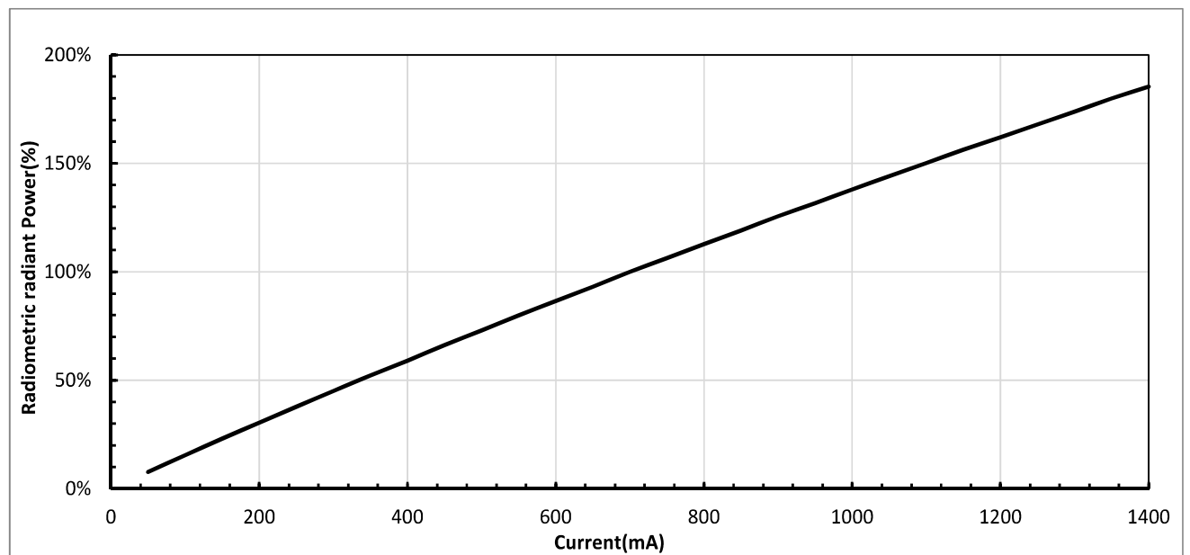
Figure 2: Relative Total Radiant Photometric vs. Drive Current ( T_{sp}=25^{\circ}\text{C} )
