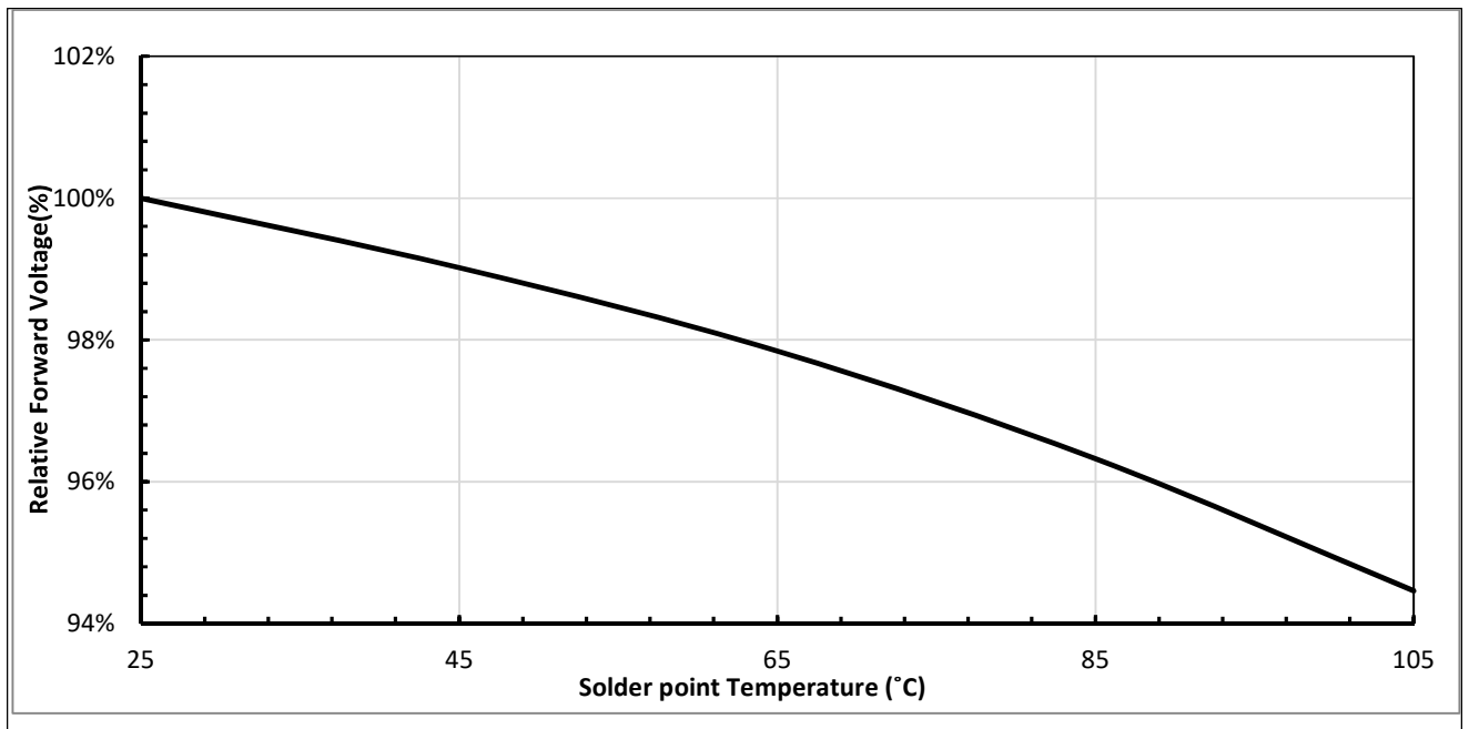
Figure 4: Forward Voltage vs. Solder Point Temperature
