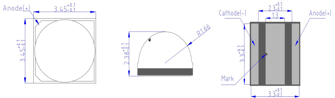
Figure 8: Drawing for SMD 3535
