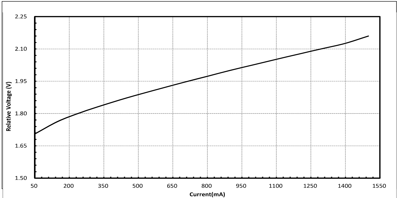
Figure 1: Drive Current vs. Relative Voltage ( T_{sp}=25^{\circ}\text{C} )
