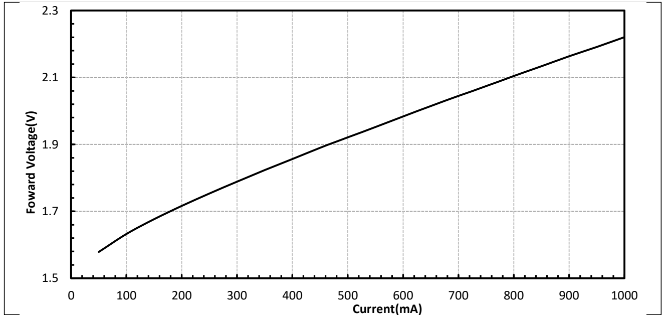
Figure 1: Drive Current vs. Voltage ( T_{sp}=25^{\circ}\text{C} )
