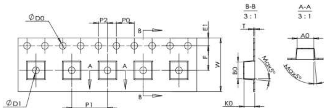
Figure 11: Emitter Tape Drawings
