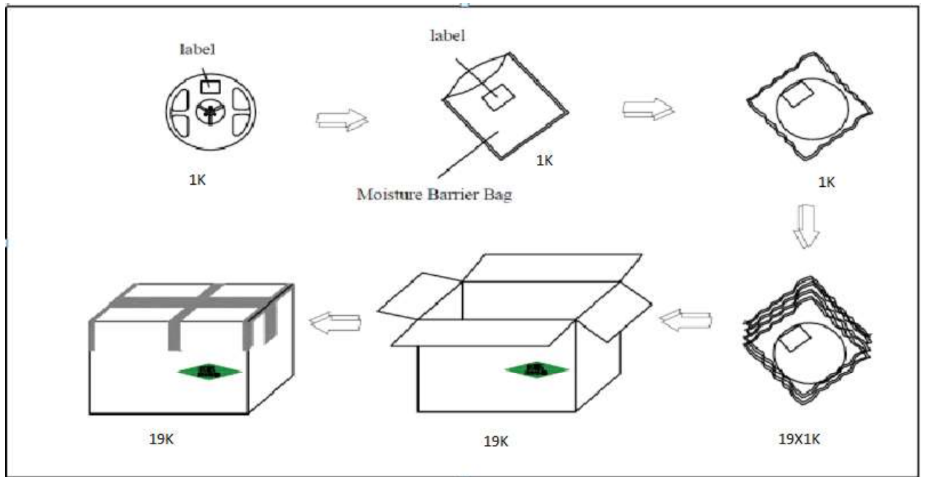
Figure 12: Emitter Reel Packaging Drawings
