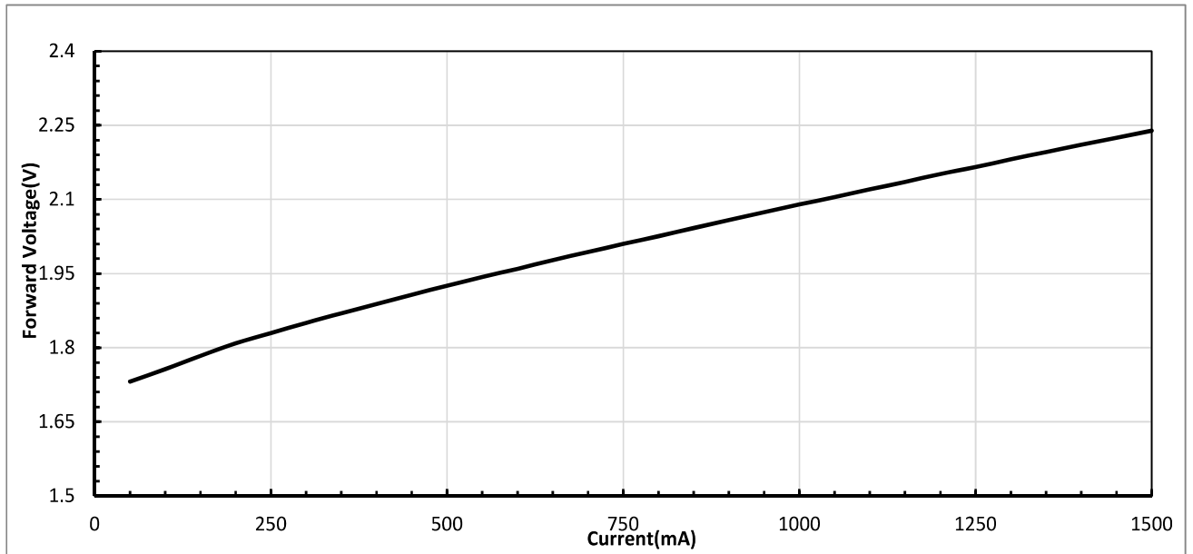
Figure 1: Drive Current vs. Forward Voltage ( T_{sp}=25^{\circ}\text{C} )
