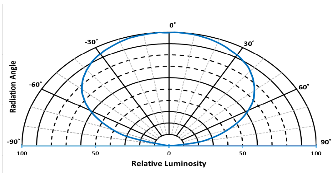
Figure 6: Typical Polar Radiation Pattern at 700mA, T_{sp}=25^{\circ}\text{C}
