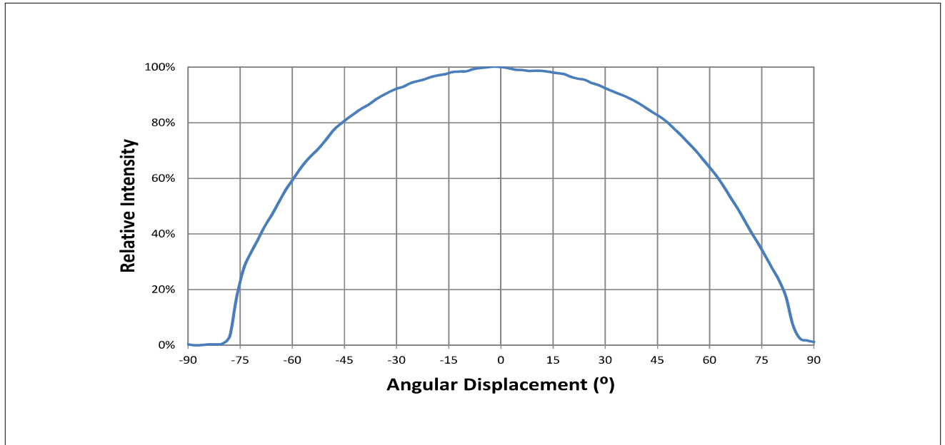
Figure 5: Typical Spatial Radiation Pattern at 700mA, T_{sp}=25^{\circ}\text{C}
