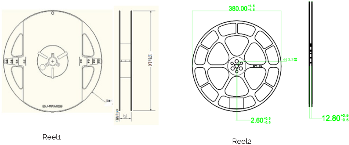
Figure 13: Emitter Reel Drawings
