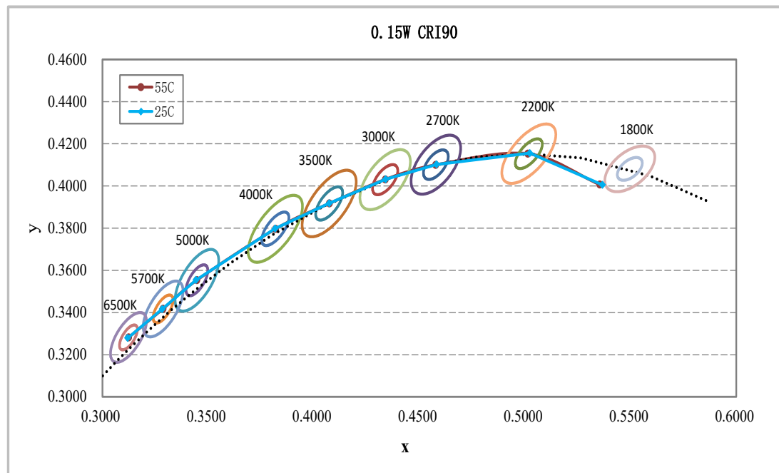
Figure 5: Chromaticity Coordinate Group (Color Targeted at T_{sp}=25^{\circ}\text{C} & 55^{\circ}\text{C} )
