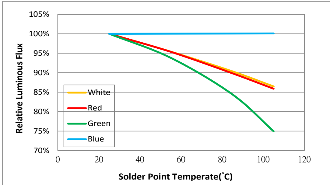
Figure 4: Typical Relative Flux vs. Solder Point Temperature_15mA
