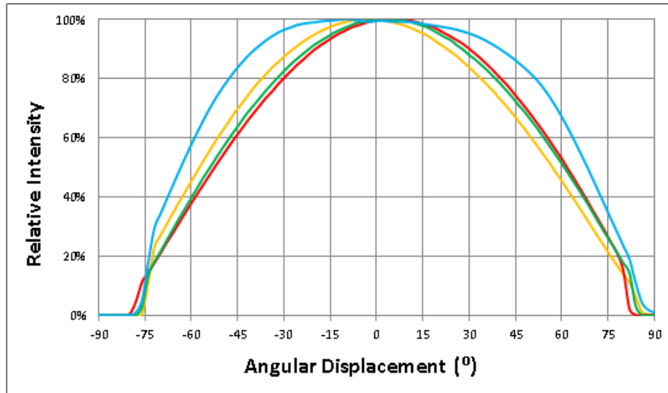
Figure 7: Typical Spatial Radiation Pattern at 15mA, T_{ca}=25^{\circ}\text{C}
