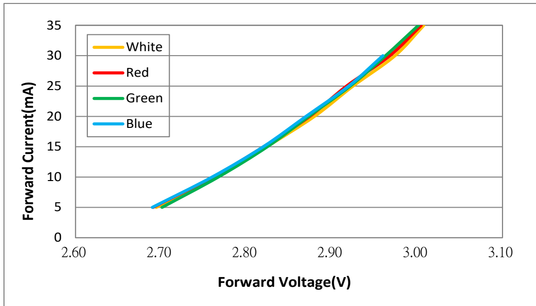
Figure 2: Drive Current vs. Voltage ( T_{sp}=25^{\circ}\text{C} )
