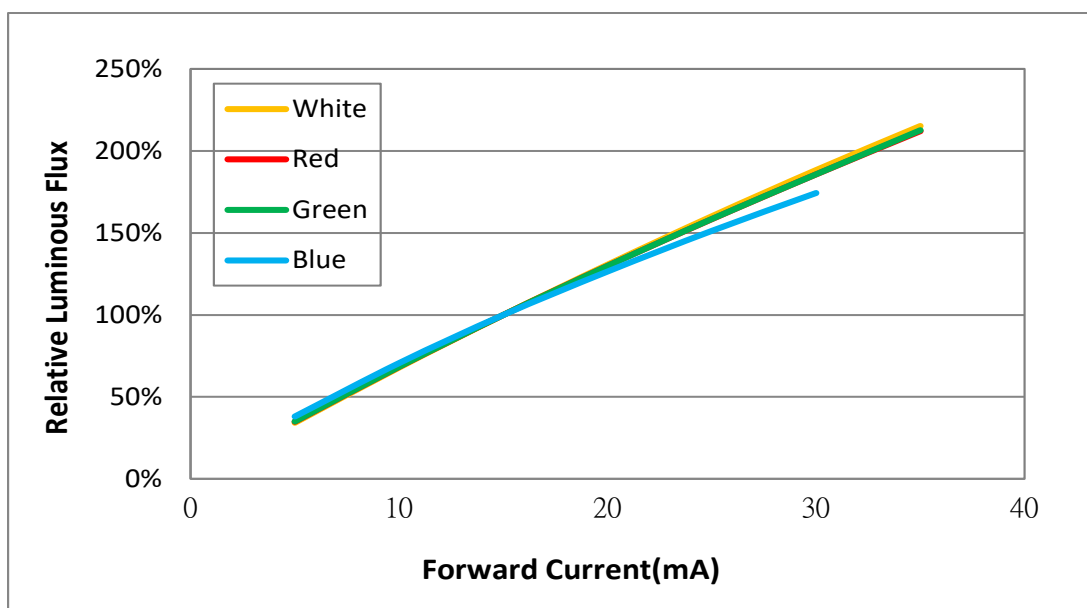
Figure 3: Typical Relative Luminous Flux vs. Drive Current ( T_{sp}=25^{\circ}\text{C} )
