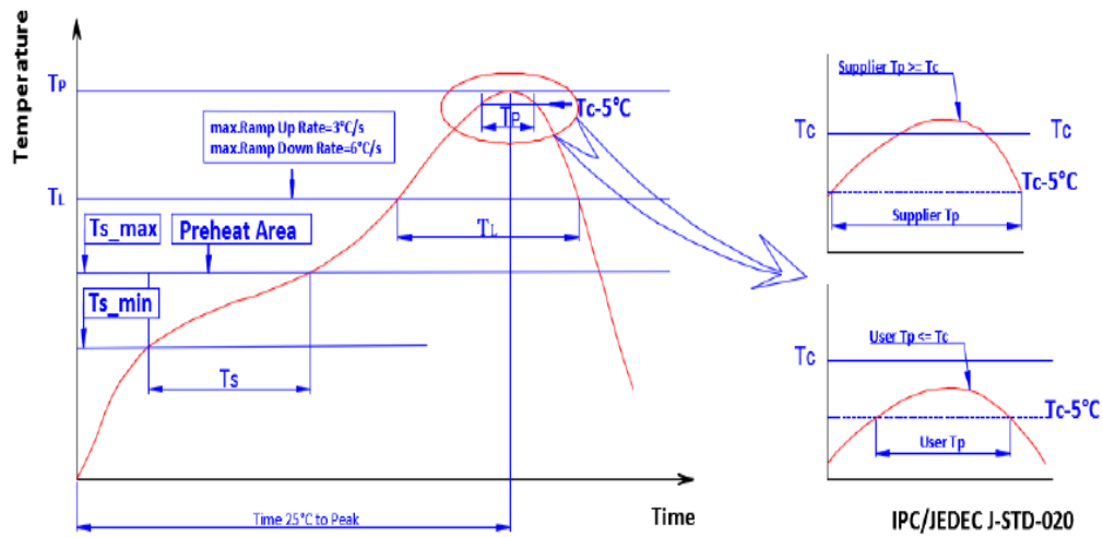
Figure 12: Reflow Profile
