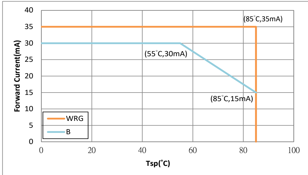
Figure 6: Drive Current vs Solder Point Temperature
