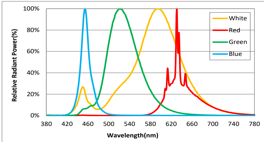
Figure 9: Typical Color Spectrum at 15mA, Tsp=25°C
