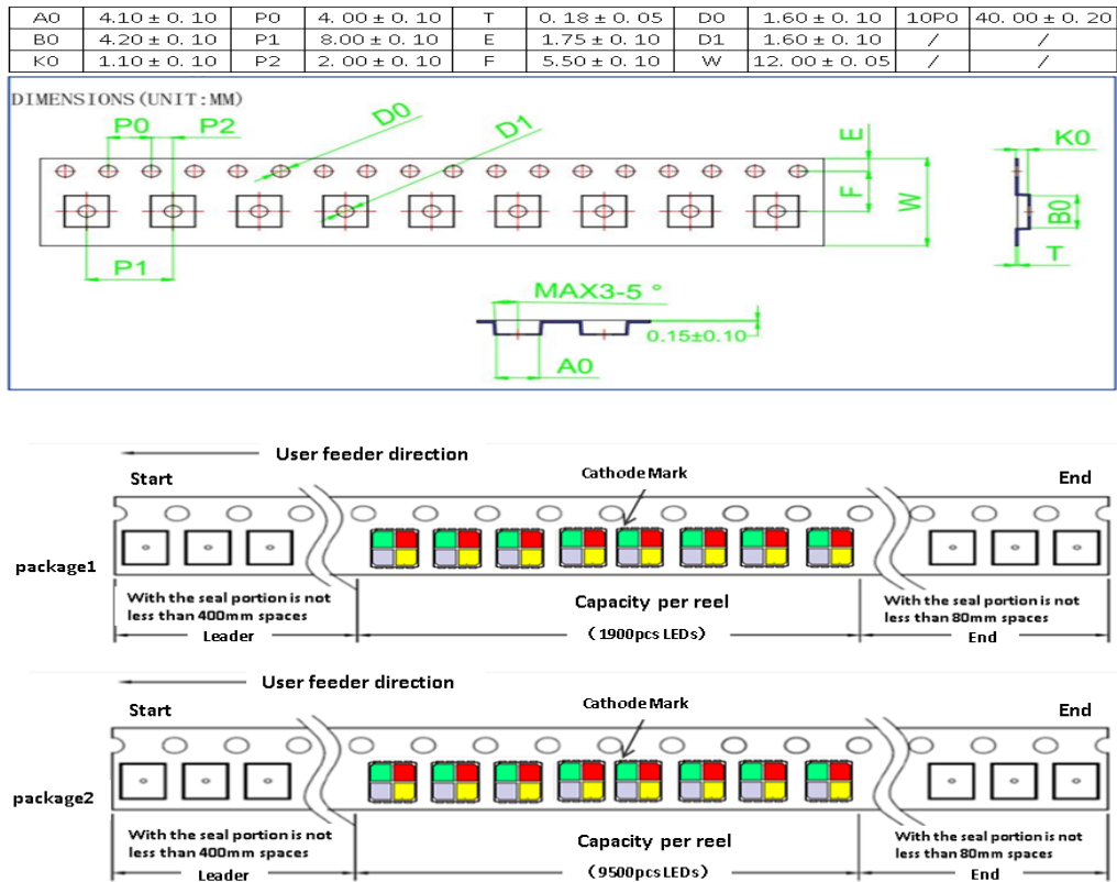
Figure 14: Emitter Tape Drawings
