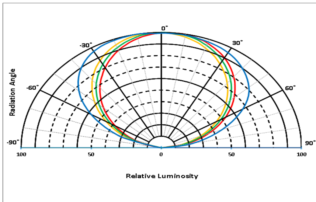
Figure 8: Typical Polar Radiation Pattern at 15mA, T_{sp}=25^{\circ}\text{C}
