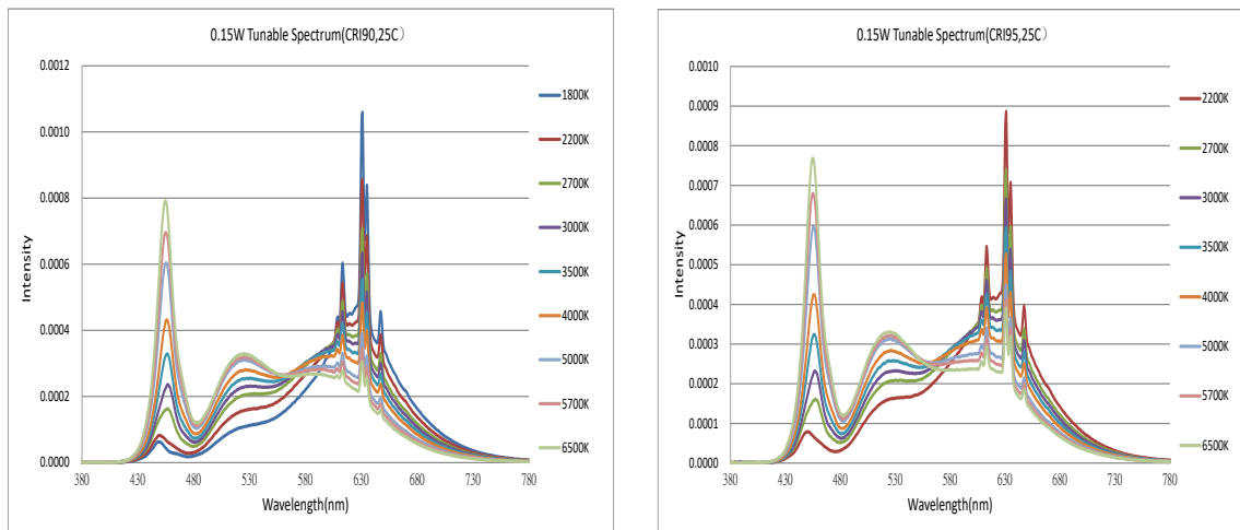
Figure 10: Tunable White Spectrum, Tsp=25°C
