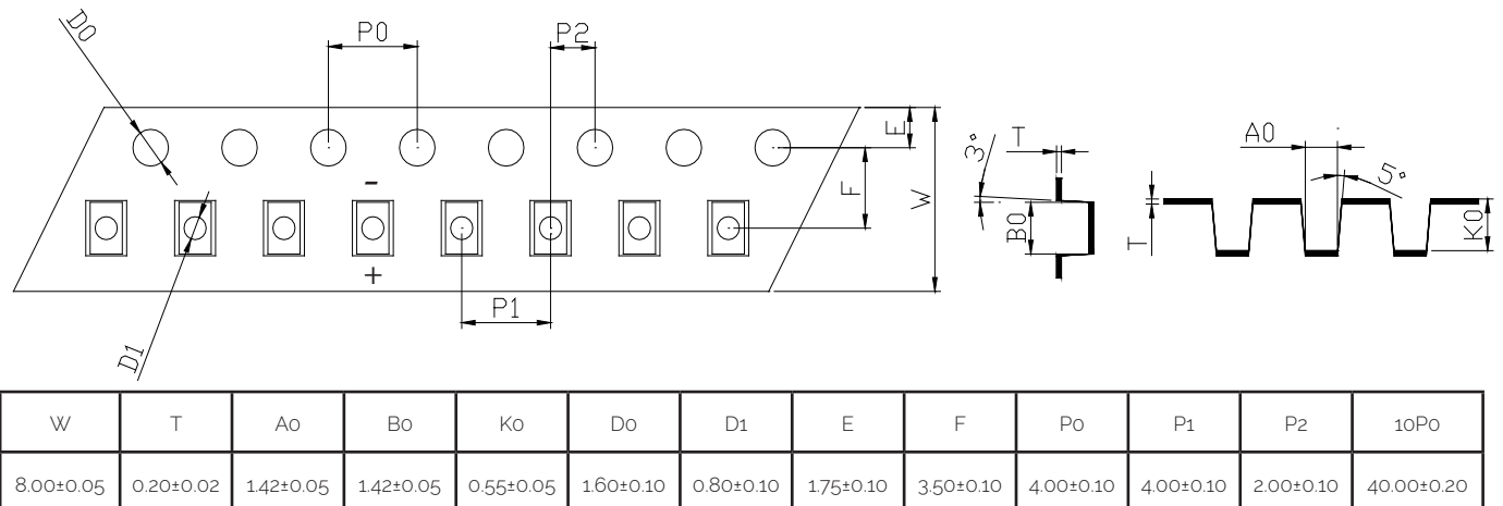
Figure 14: Tape Drawings
