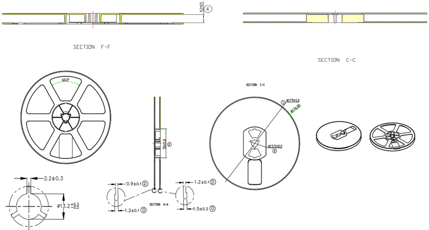
Figure 13: Reel Drawings
