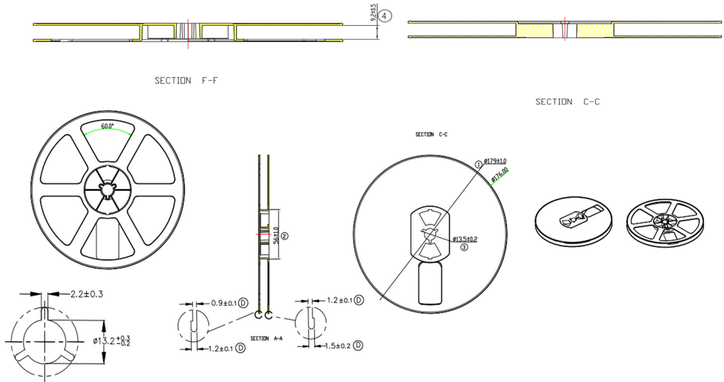
Figure 13: Reel Drawings
