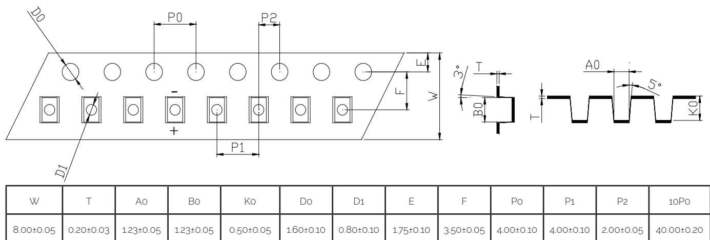
Figure 14: Tape Drawings
