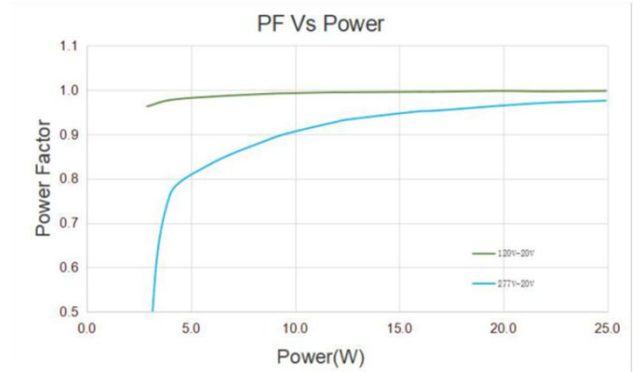
Figure 4: Power Factor vs. Output Power
