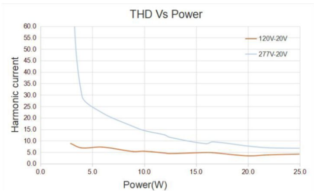
Figure 5: THD vs Output Power
