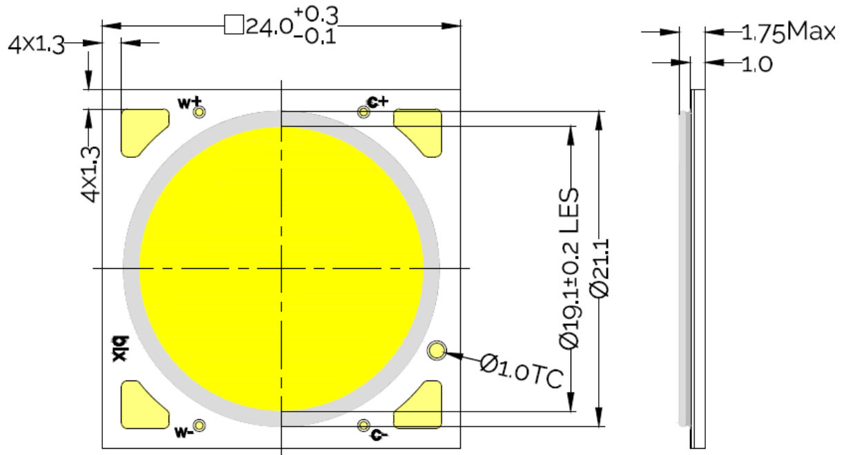
Figure 19: Mechanical Drawing Specifications BXRV-TR-XXXXX-40Ax-A-3X
