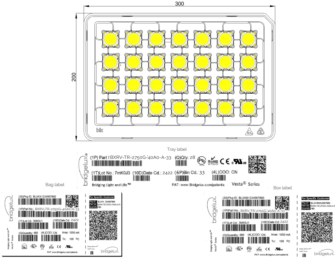
Figure 22: Vesta Series Tunable White Gen 3 18mm Packaging and Labeling
