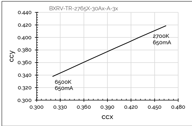
Figure 7: CCT Tuning Range, Tc=85°C
