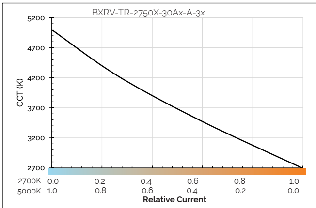
Figure 9: CCT vs. Relative Warm White Current
