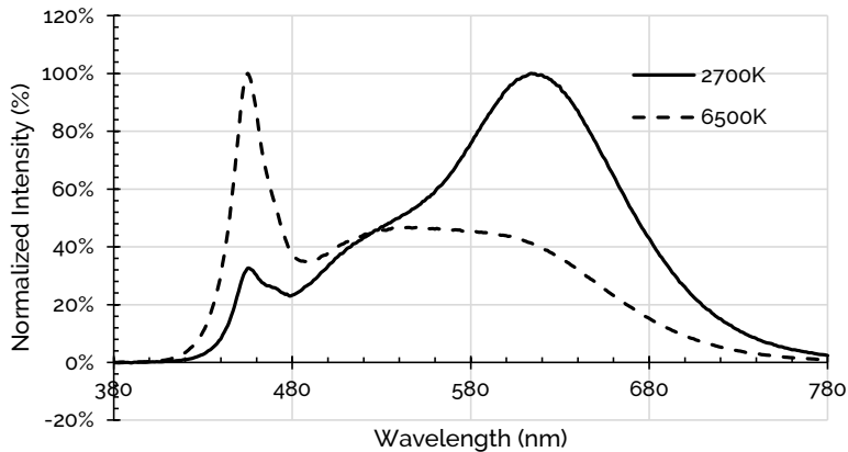
Figure 18: 2700K - 6500K with 90 CRI , 85°C
