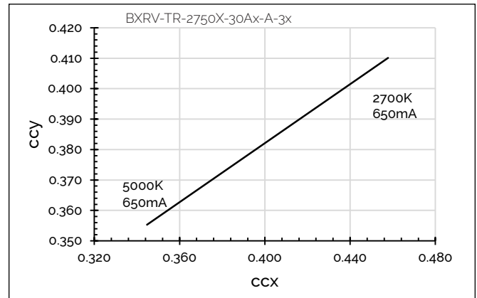
Figure 6: CCT Tuning Range, T_c=85^\circ\text{C}
