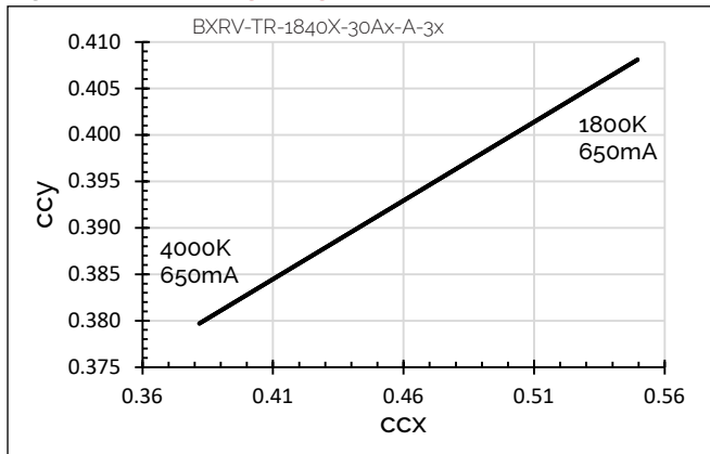
Figure 5: CCT Tuning Range, T_c=85^\circ\text{C}
