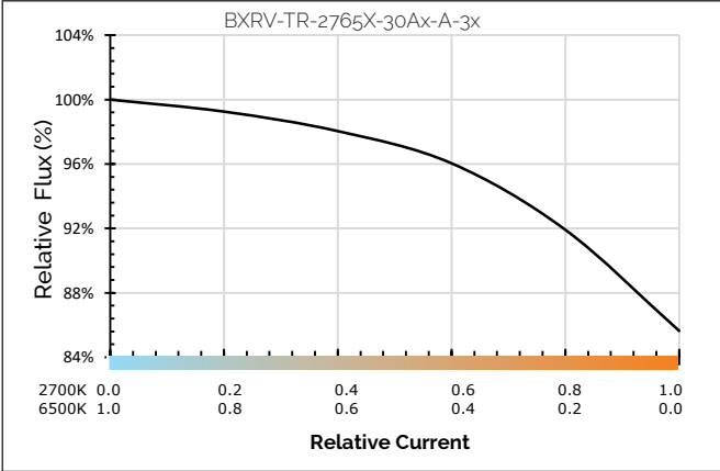
Figure13: Relative Flux vs. Relative Current
