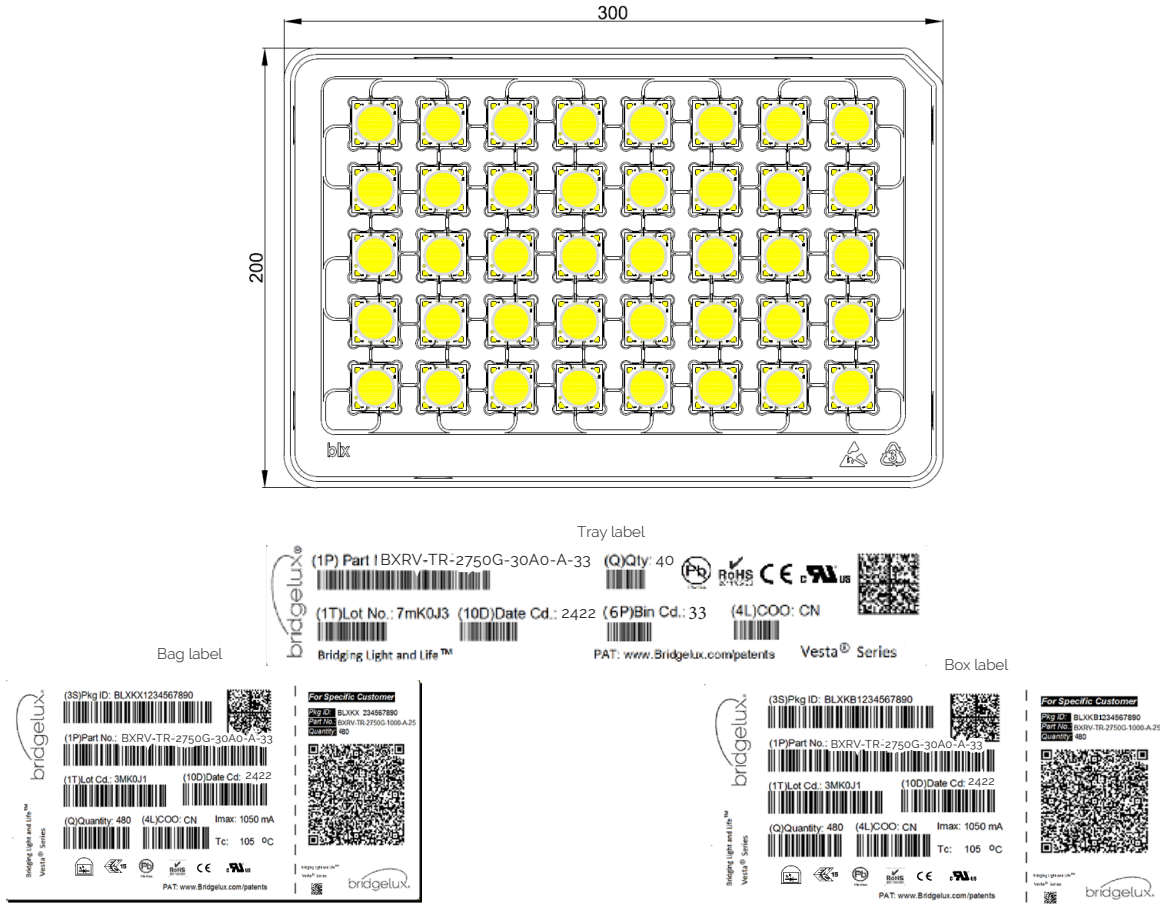
Figure 22: Vesta Series Tunable White Gen 3 15mm Packaging and Labeling
