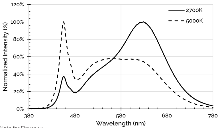
Figure 17: 2700K - 5000K with 90 CRI , 85°C
