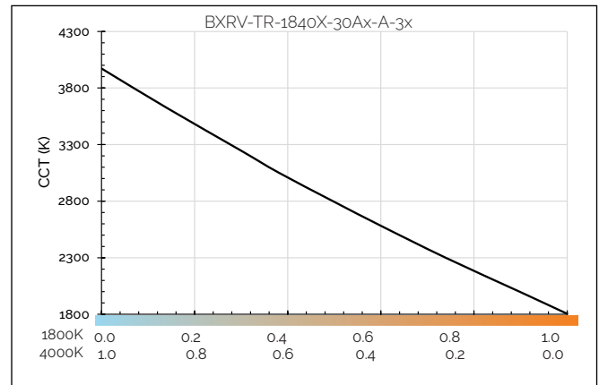
Figure 8: CCT vs. Relative Warm White Current
