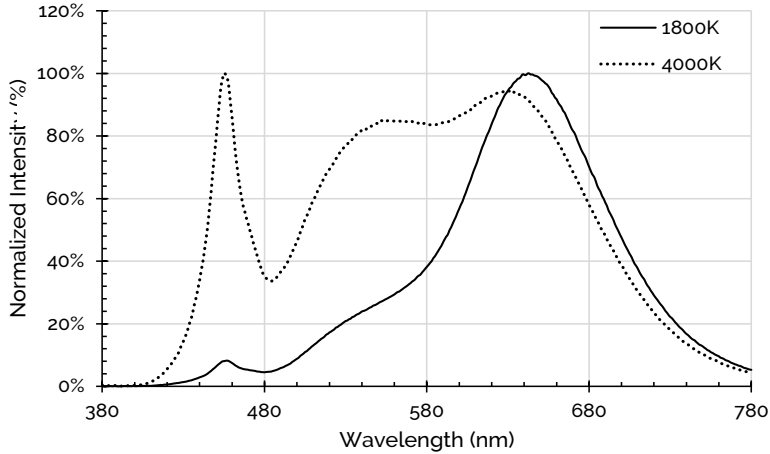
Figure 16: 1800K - 4000K with 90 CRI , 85°C
