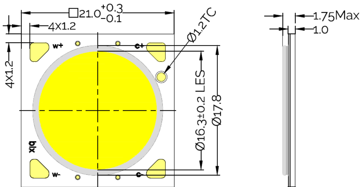
Figure 19: Mechanical Drawing Specifications BXRV-TR-XXXXX-30Ax-A-3X
