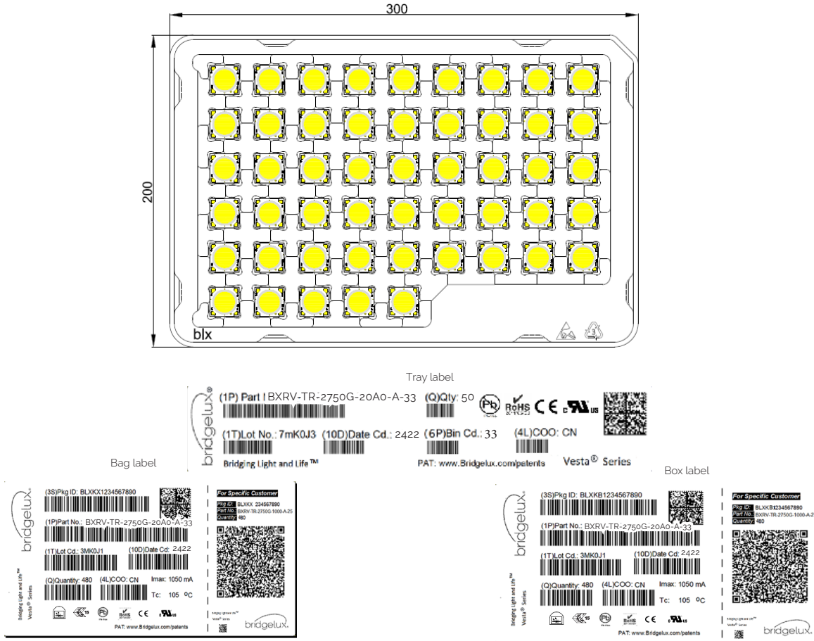
Figure 22: Vesta Series Tunable White Gen 3 13mm Packaging and Labeling
