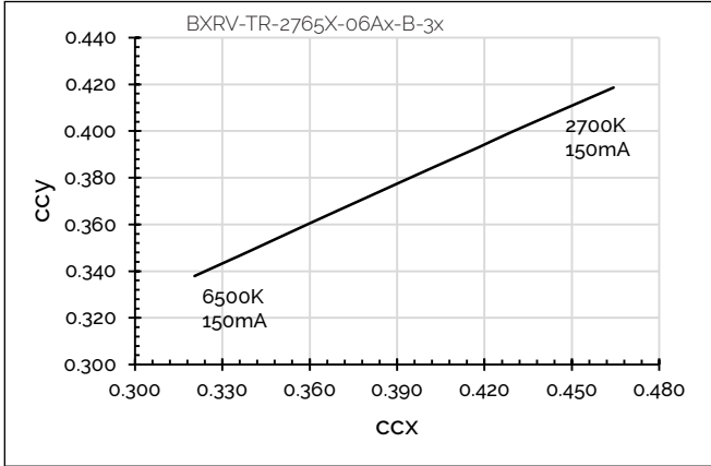
Figure 7: CCT Tuning Range, Tc=85°C
