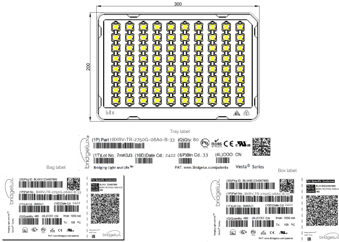
Figure 22: Vesta Series Tunable White Gen 3 6mm Packaging and Labeling
