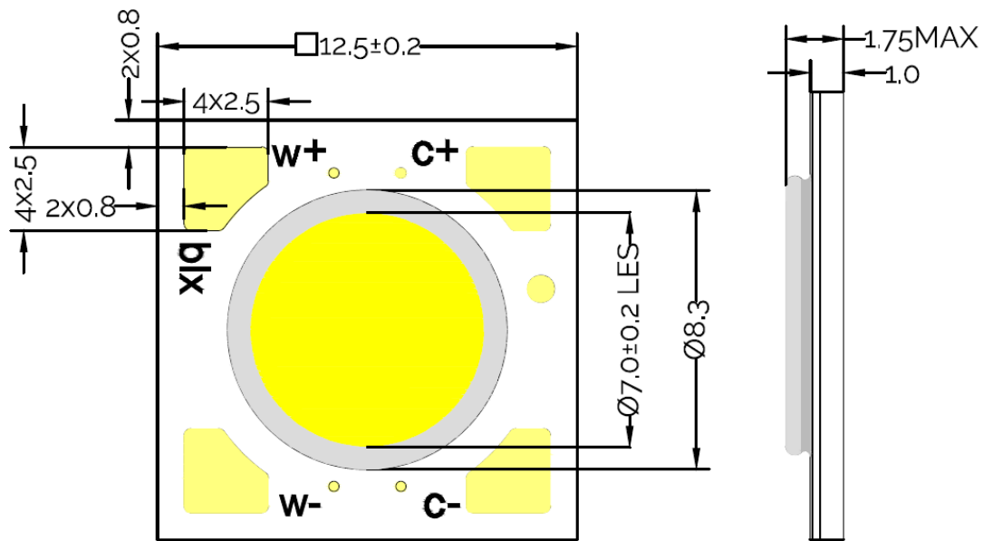
Figure 19: Mechanical Drawing Specifications BXRV-TR-XXXXX-06Ax-B-3X
