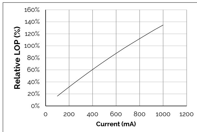
Figure 2: VgE HD Typical Relative Flux vs. Drive Current ( T_j = T_c = 25^\circ\text{C} ) 1
