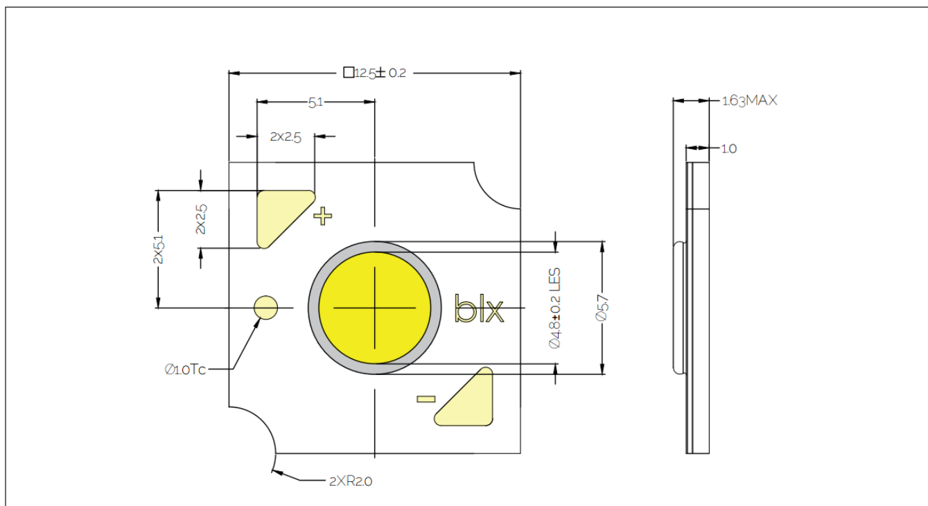
Figure 12: Drawing for V4 HD LED Array
