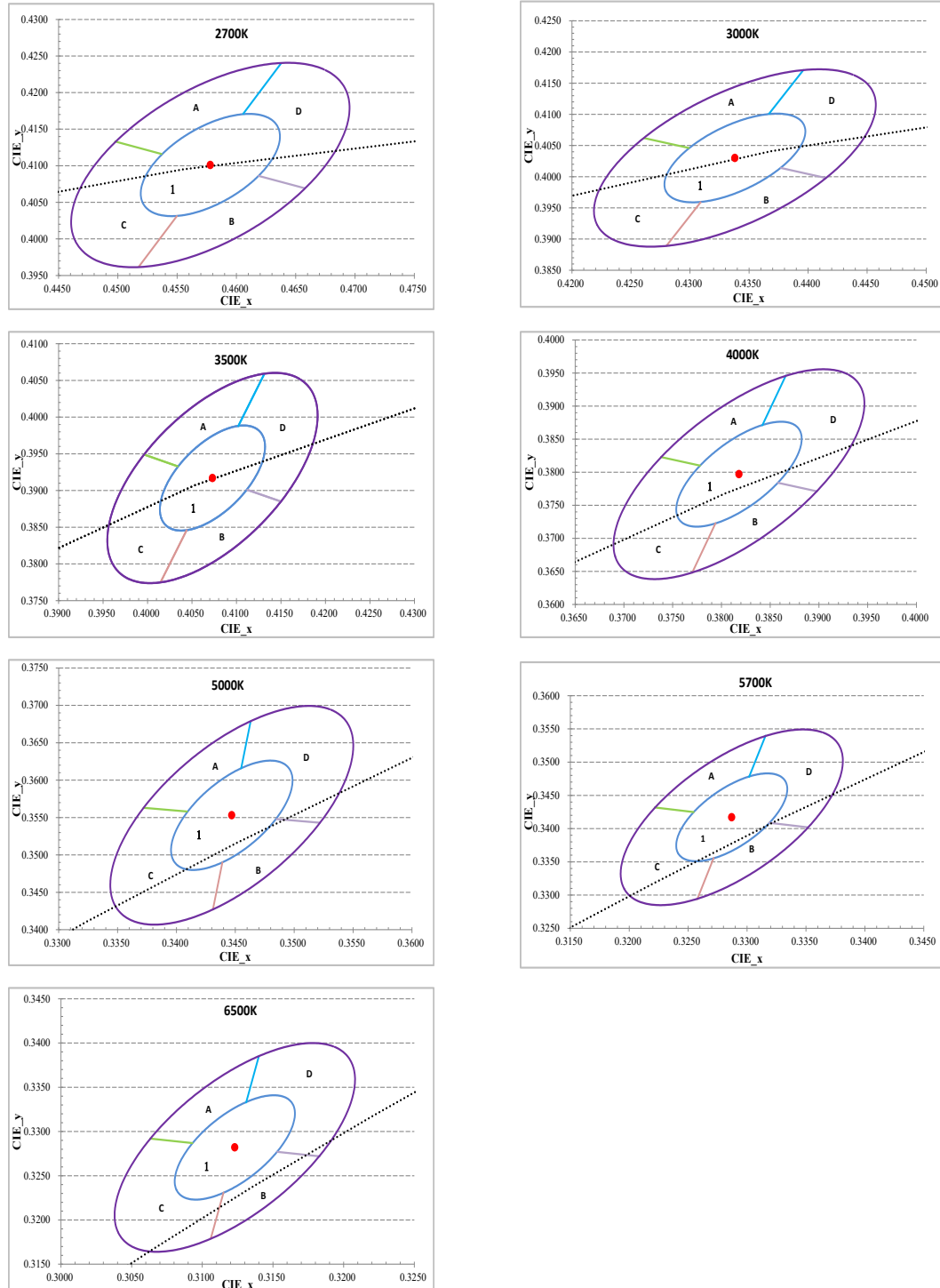
Figure 1: C.I.E. 1931 Chromaticity Diagram ( Hot-color Targeted at T_{sp}=60^{\circ}\text{C} )
