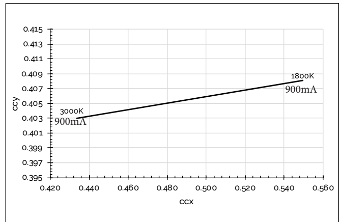
Figure 15: CCT Tuning Range, T_c=85^\circ\text{C}
