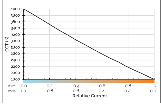
Figure 13: CCT vs. Relative Current, T_c=85^\circ\text{C}
