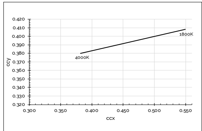
Figure 17: CCT Tuning Range, T_c=85^\circ\text{C}
