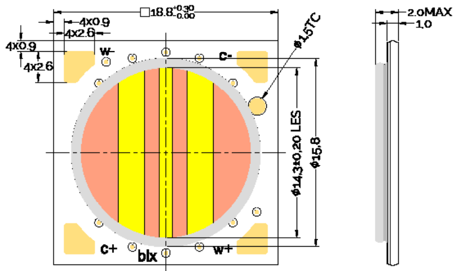
Figure 28: Drawing for Vesta Series Tunable White Gen 2 13mm Array
