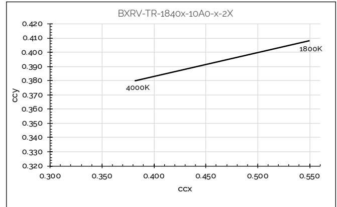
Figure 29: CCT Tuning Range, Tc=85°C
