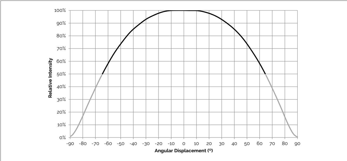
Figure 31: Typical Spatial Radiation Pattern
