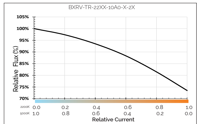
Figure 23: Relative Flux vs. Relative Current
