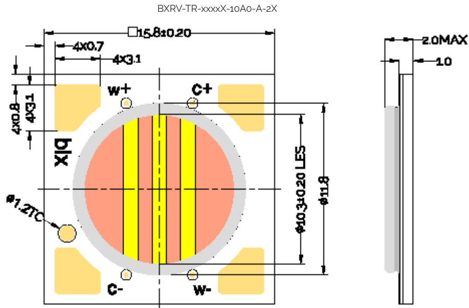
Figure 42: Drawing for Vesta Series Tunable White Gen2 9mm, 18V Array
