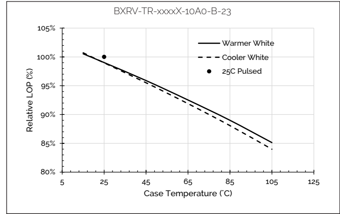
Figure 13: Relative Flux vs. Case Temperature
