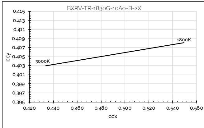
Figure 28: CCT Tuning Range, Tc=85°C
