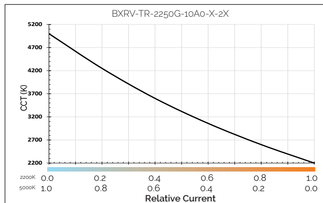
Figure 22: CCT vs. Relative Current, Tc=85°C
