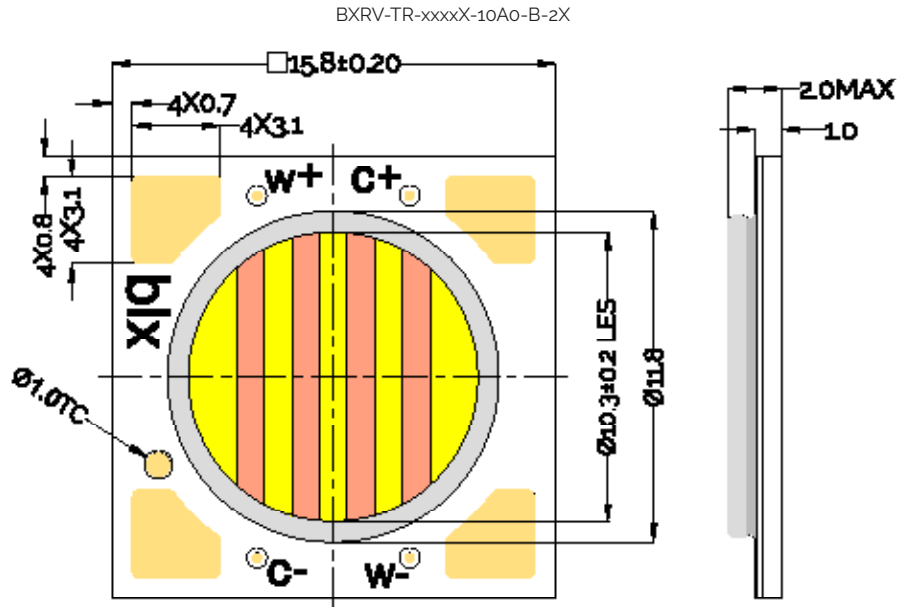
Figure 41: Drawing for Vesta Series Tunable White Gen2 9mm, 36V Array
