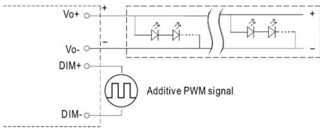
Figure 14: PWM Signal Dimming Curve and Circuitry
