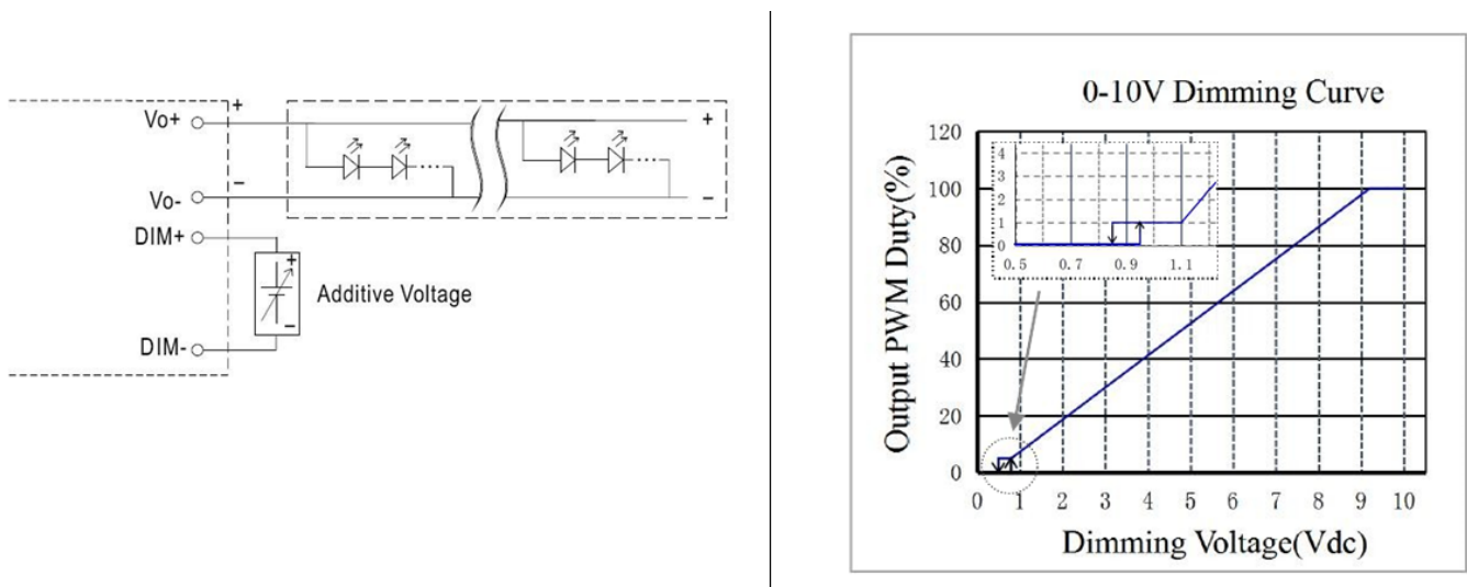
Figure 13: 1-10V Dimming Curve and Circuitry
