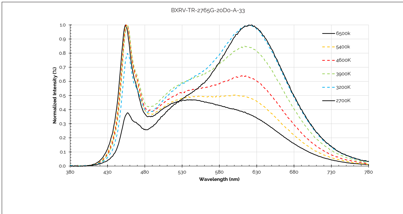
Figure 11: 2700K - 6500K with 90 CRI
