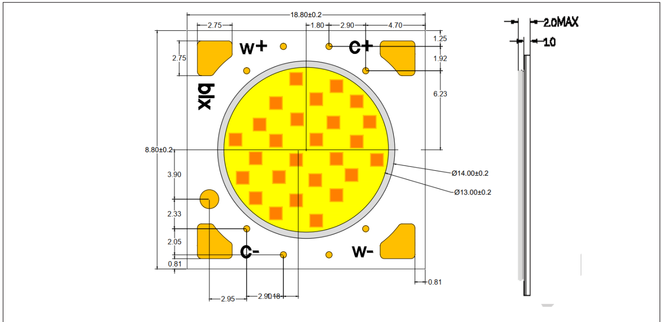
Figure 12: Mechanical Drawing Specifications
