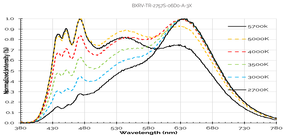
Figure 27: 2700K-5700K with Thrive
