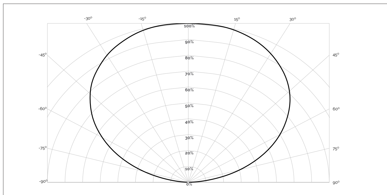
Figure 24: Typical Polar Radiation Pattern
