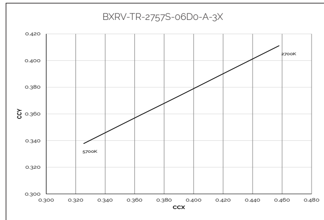
Figure 21: CCT Tuning Range, Tc=85C
