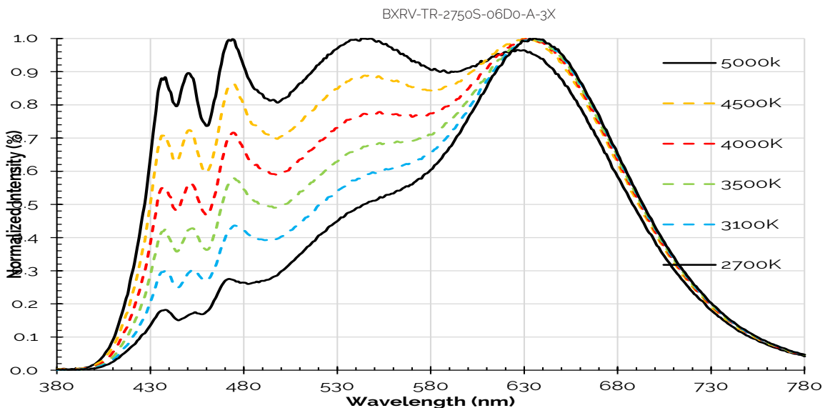
Figure 26: 2700K-5000K with Thrive
