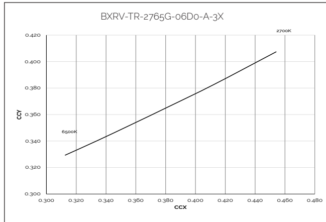
Figure 19: CCT Tuning Range, Tc=85C
