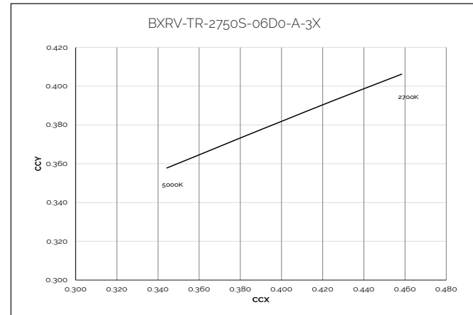
Figure 20: CCT Tuning Range, Tc=85C
