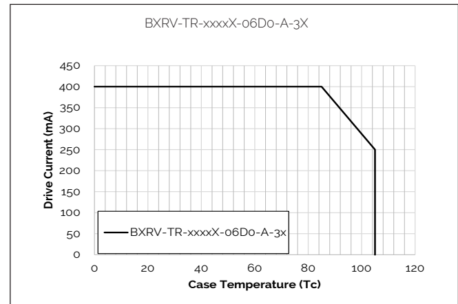
Figure 22: Derating Curve
