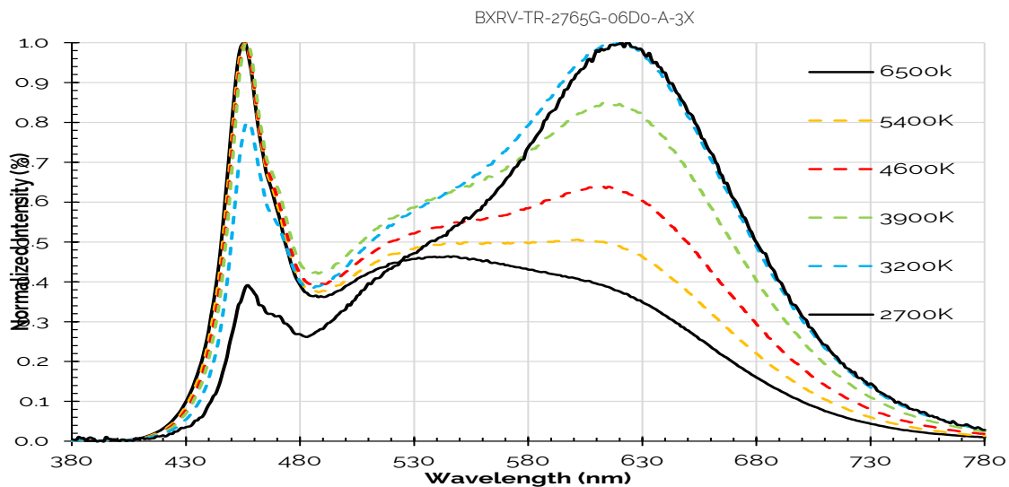
Figure 25: 2700K-6500K with CRI90
