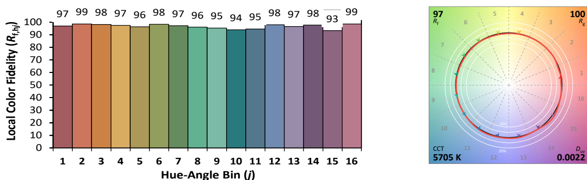
Figure 3: 5700K Thrive TM-30 Graphs at T_c=85^\circ\text{C}
