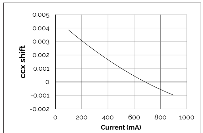
Figure 10: V6G HD Drive Current vs. ccx Shift
