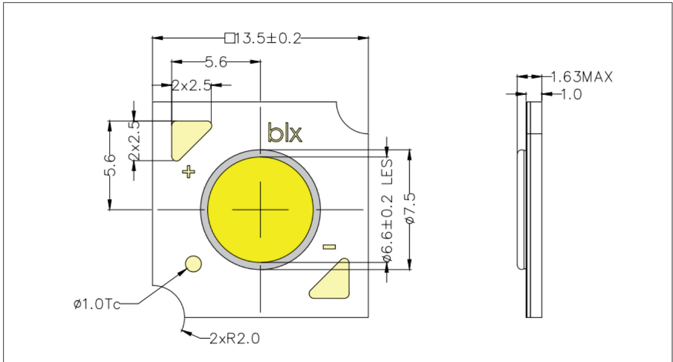
Figure 15: Drawing for V6 HD LED Array
