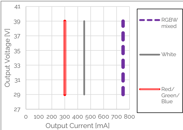
Figure 1: Operating Window
