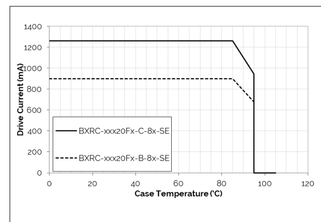
Figure 6: Derating Curve
