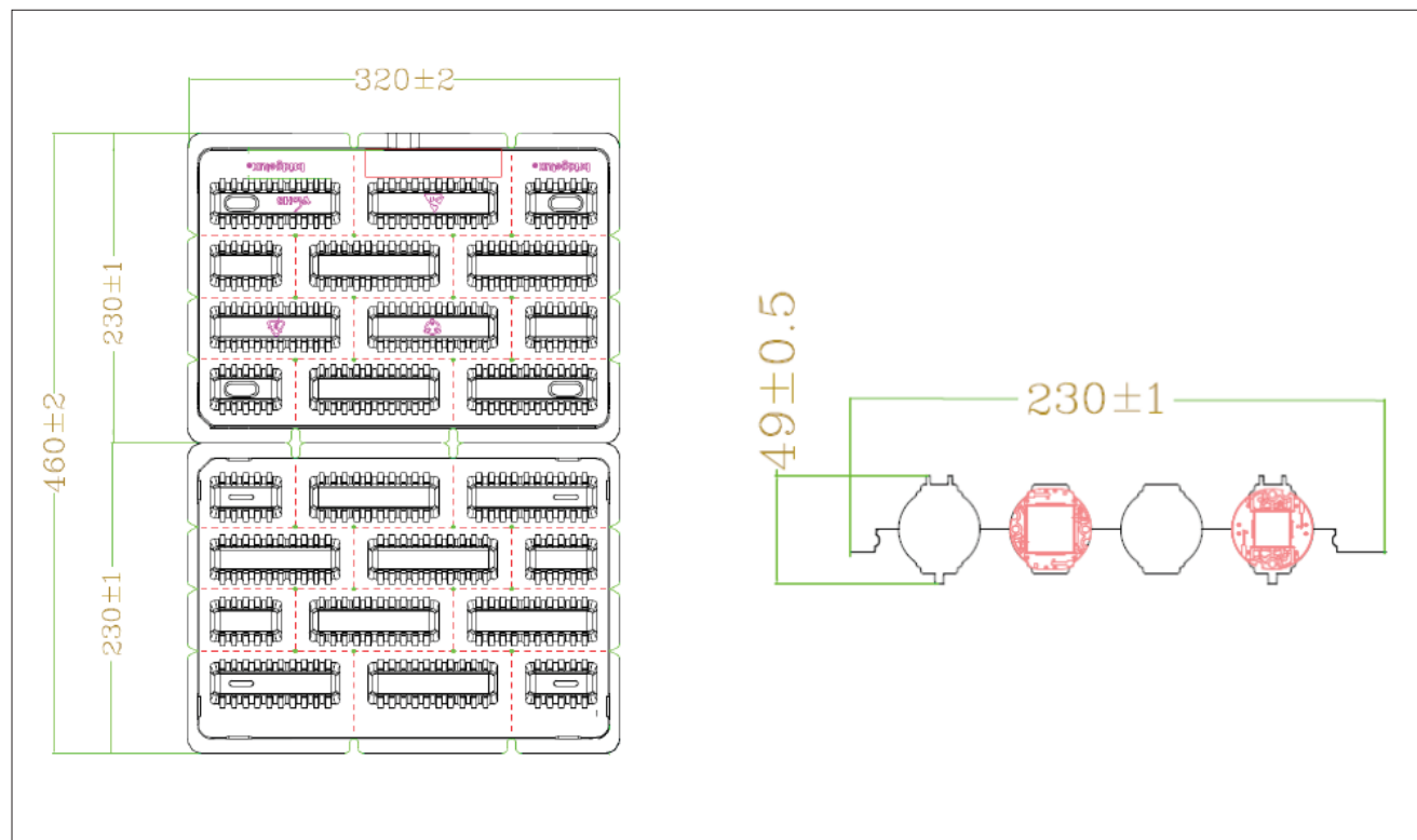
Figure 19: Drawing for Vero SE 18 Packaging Tray
