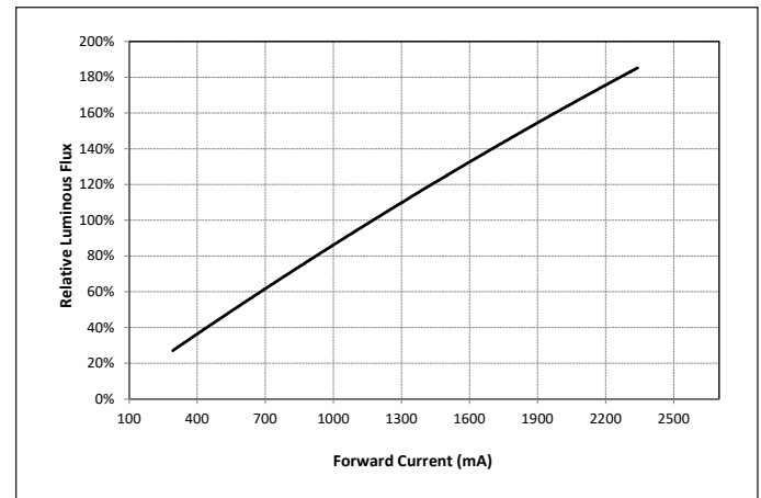
Figure 12: Vero SE 18C Typical Relative Flux vs. Current ( T_c = 25^\circ\text{C} )
