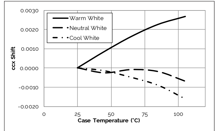
Figure 14: Typical cxc Shift vs. Case Temperature
