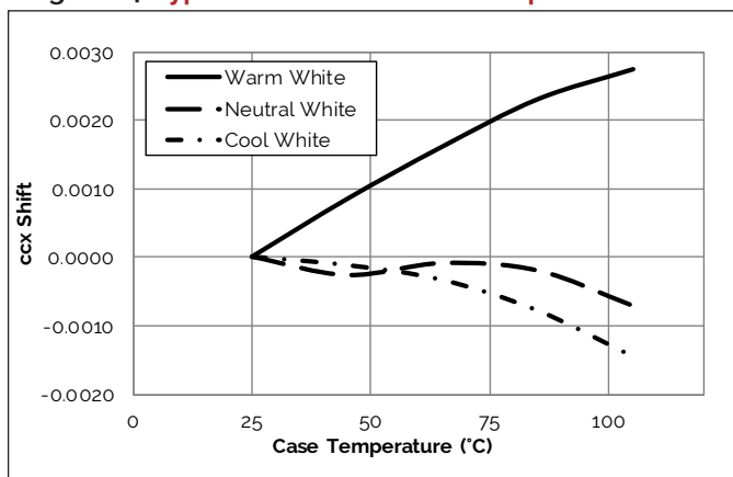
Figure 14: Typical ccx Shift vs. Case Temperature
