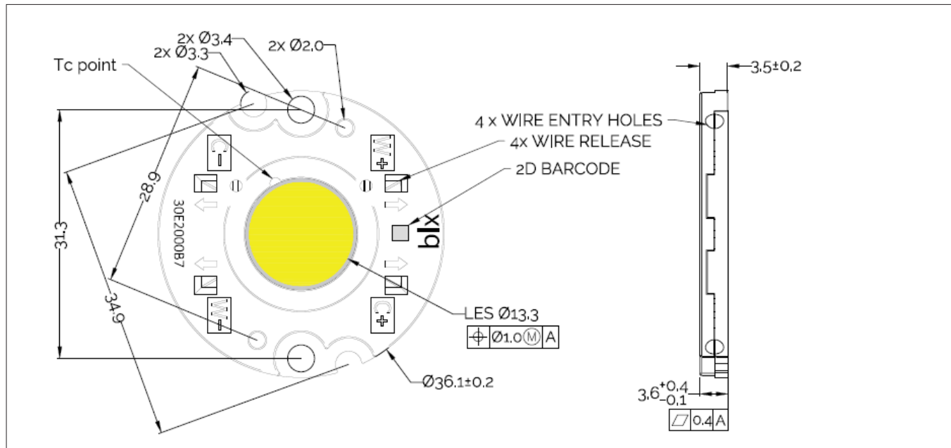
Figure 18: Drawing for Vero SE 13 LED Array
