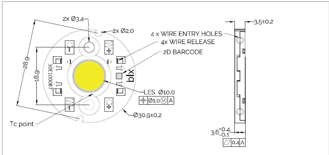
Figure 22: Drawing for Vero SE 10 LED Array
