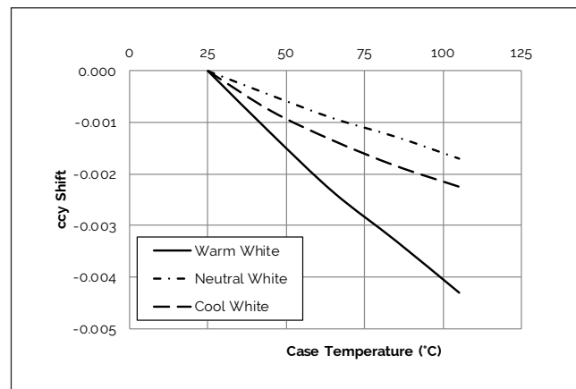
Figure 19: Typical ccy Shift vs. Case Temperature
