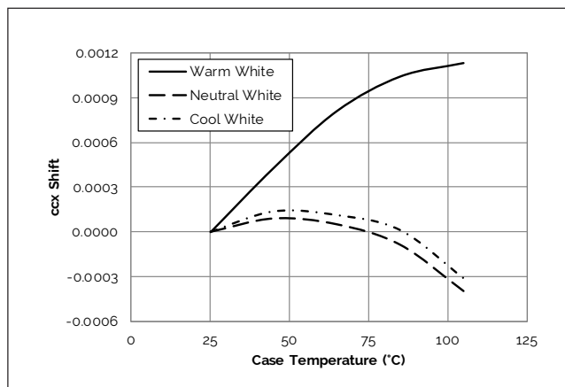
Figure 18: Typical ccx Shift vs. Case Temperature
