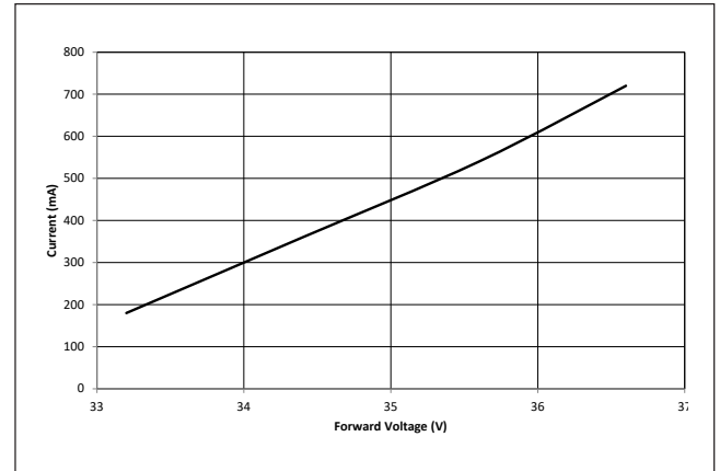
Figure 12: Vero SE 10C Drive Current vs. Voltage ( T_c=25^\circ\text{C} )
