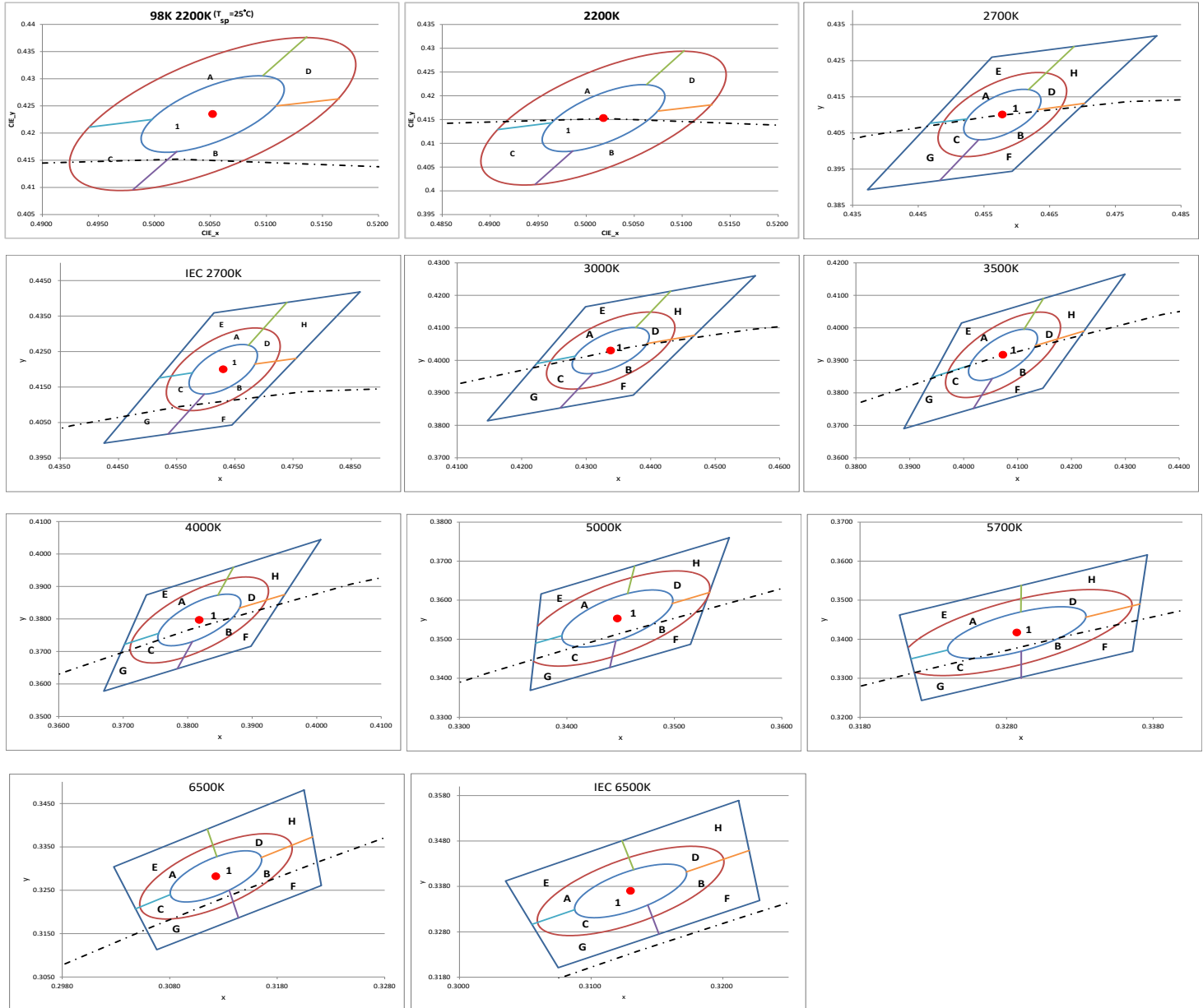
Figure 1: C.I.E. 1931 Chromaticity Diagram ( Hot-color Targeted at T_{sp}=85^{\circ}\text{C} , 98K 2200K at T_{sp}=25^{\circ}\text{C} )
