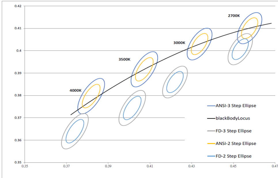
Figure 13: Warm ,Neutral White Test Bins in xy Color Space
