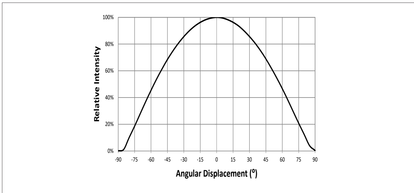
Figure 14: Typical Spatial Radiation Pattern at 100mA, T_{sp}=25^{\circ}\text{C}
