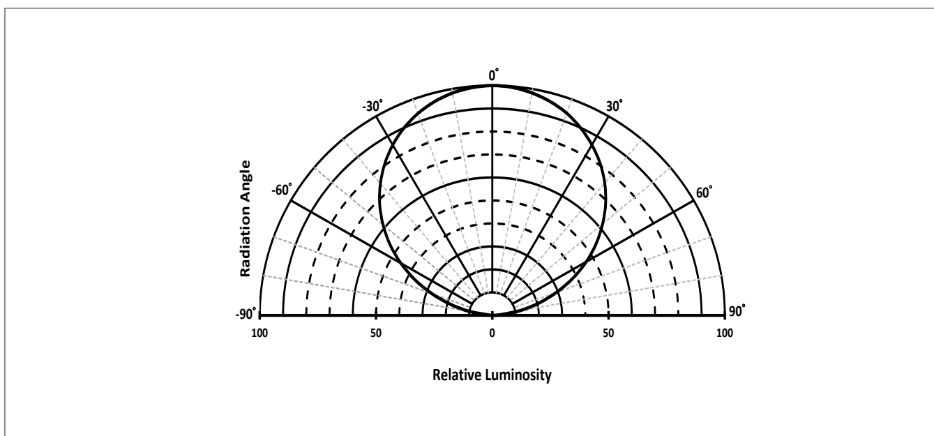
Figure 15: Typical Polar Radiation Pattern at 100mA, T_{sp}=25^{\circ}\text{C}
