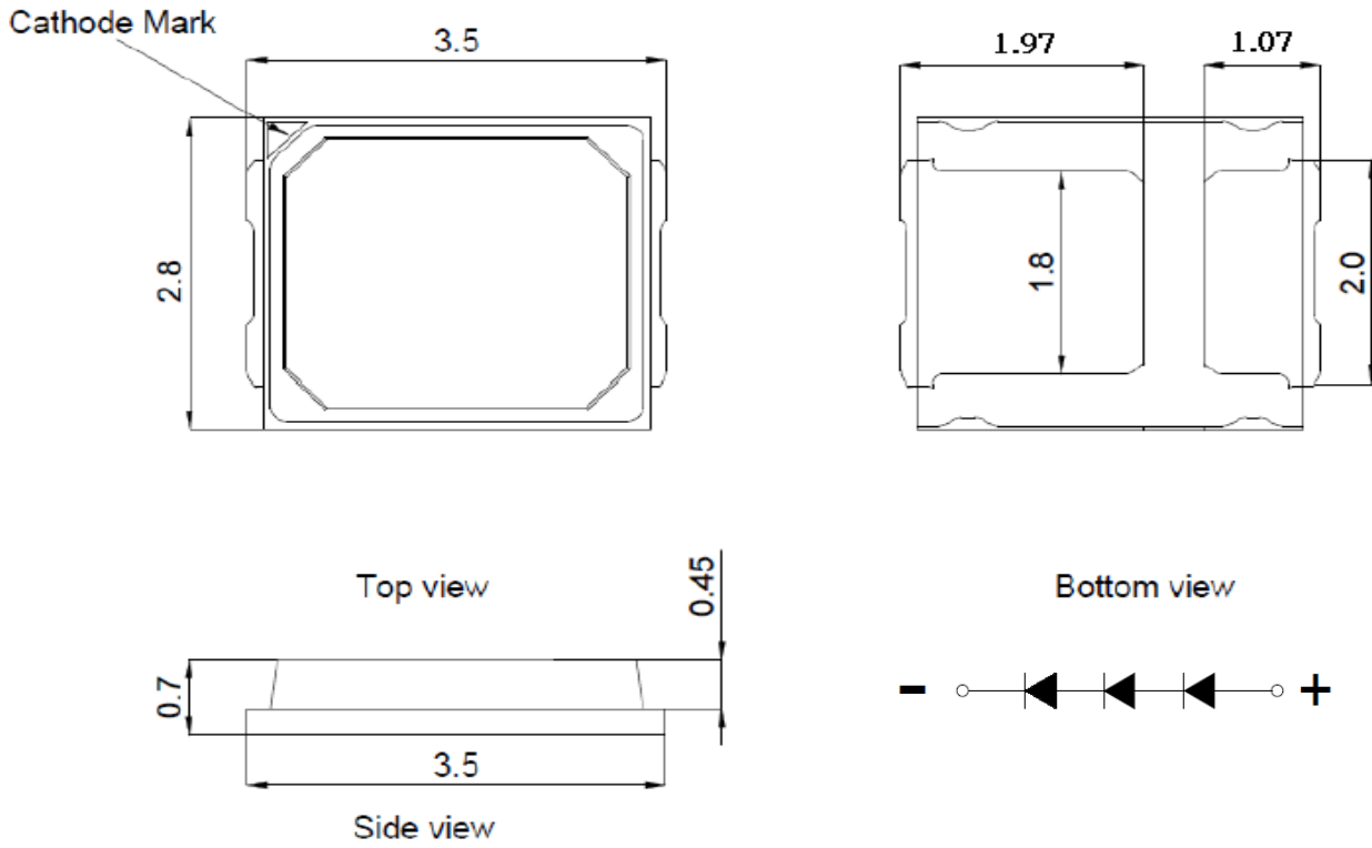
Figure 16: Drawing for SMD 2835
