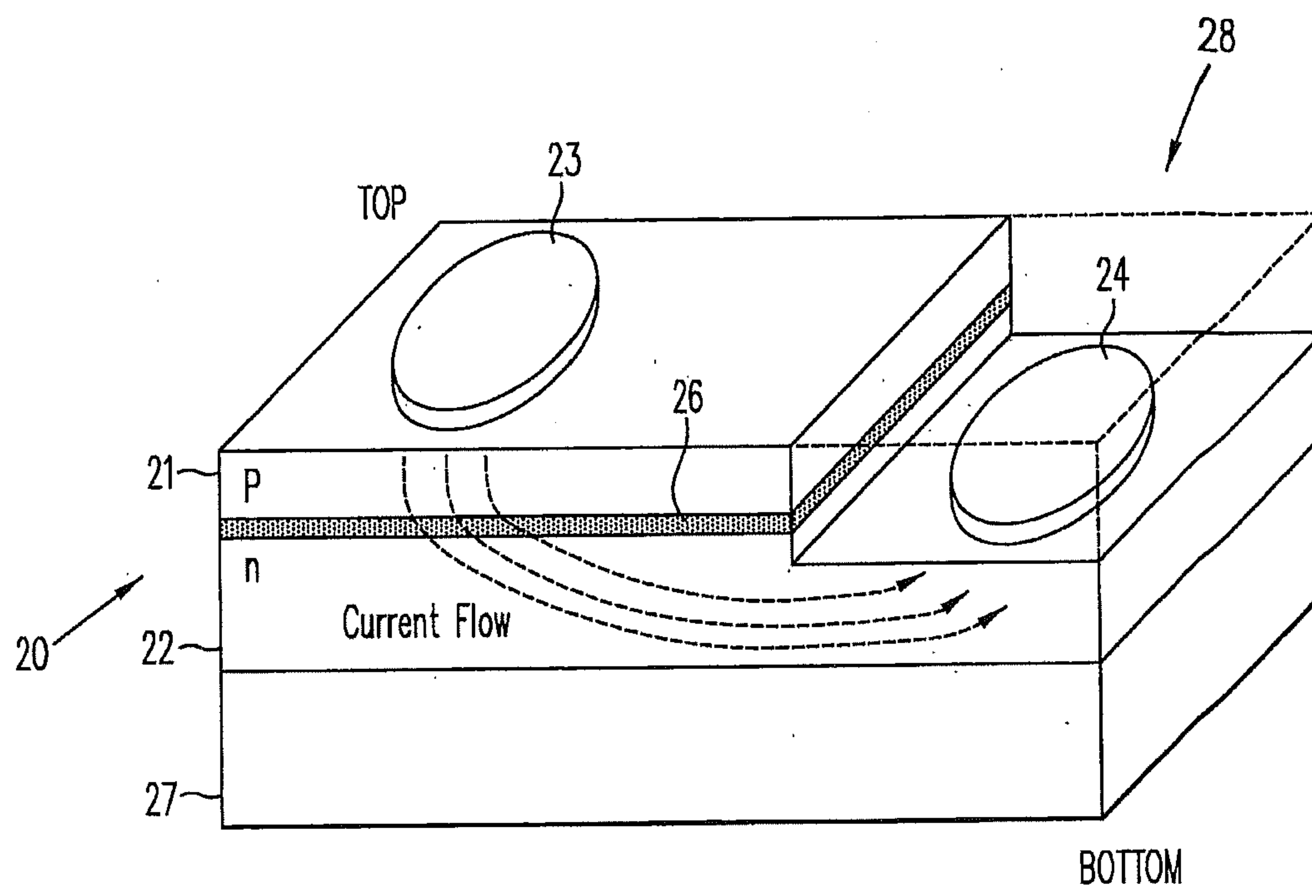
FIG. 2 (Prior Art)
