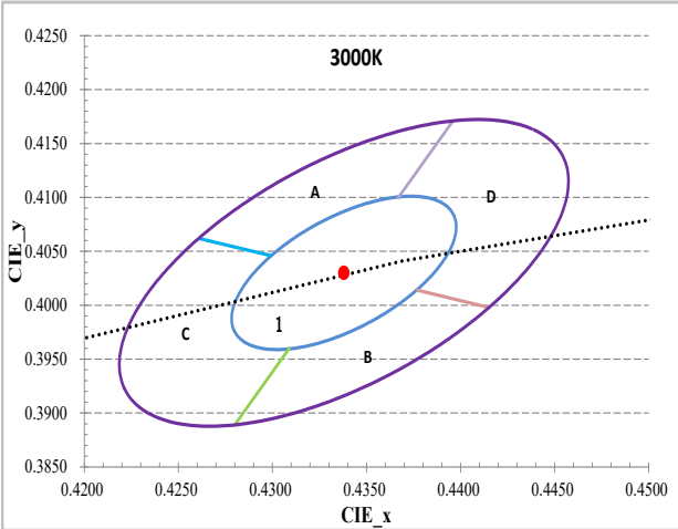
Figure 1: C.I.E. 1931 Chromaticity Diagram (5 Color Bin Structure, Hot-color Targeted at T_{sp} = 55^{\circ}\text{C} )
