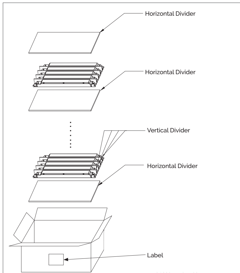
Figure 11: Packaging Box Design
