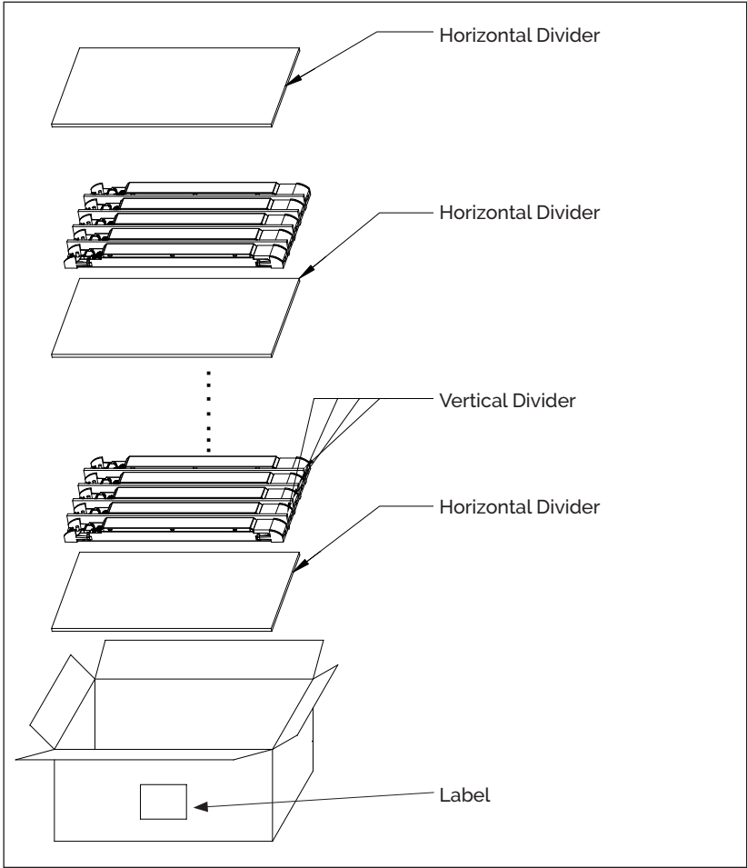
Figure 12: Packaging Box Design
