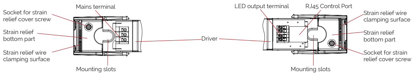
Figure 10: Strain Relief Feature Map
