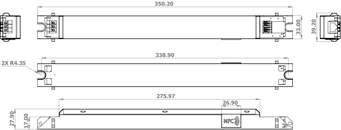
Figure 8: Mechanical Drawing
