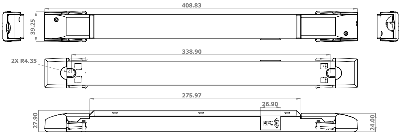
Figure 9: Mechanical Drawing for Driver With Strain Relief
