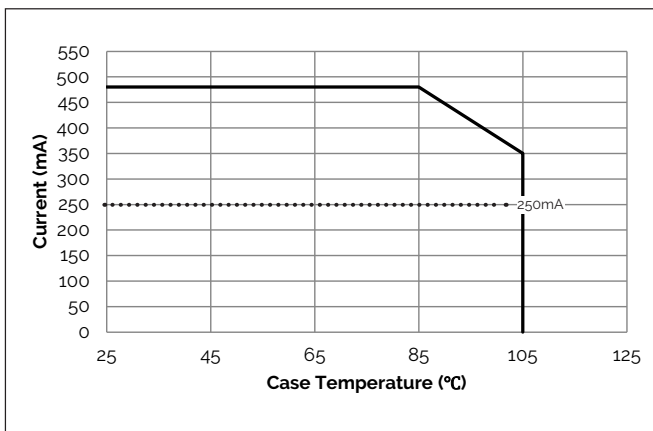
Figure 8: Derating Curve
