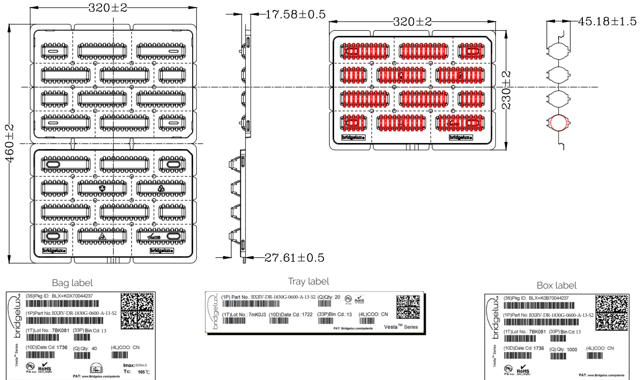
Figure 14: Packaging Specifications
