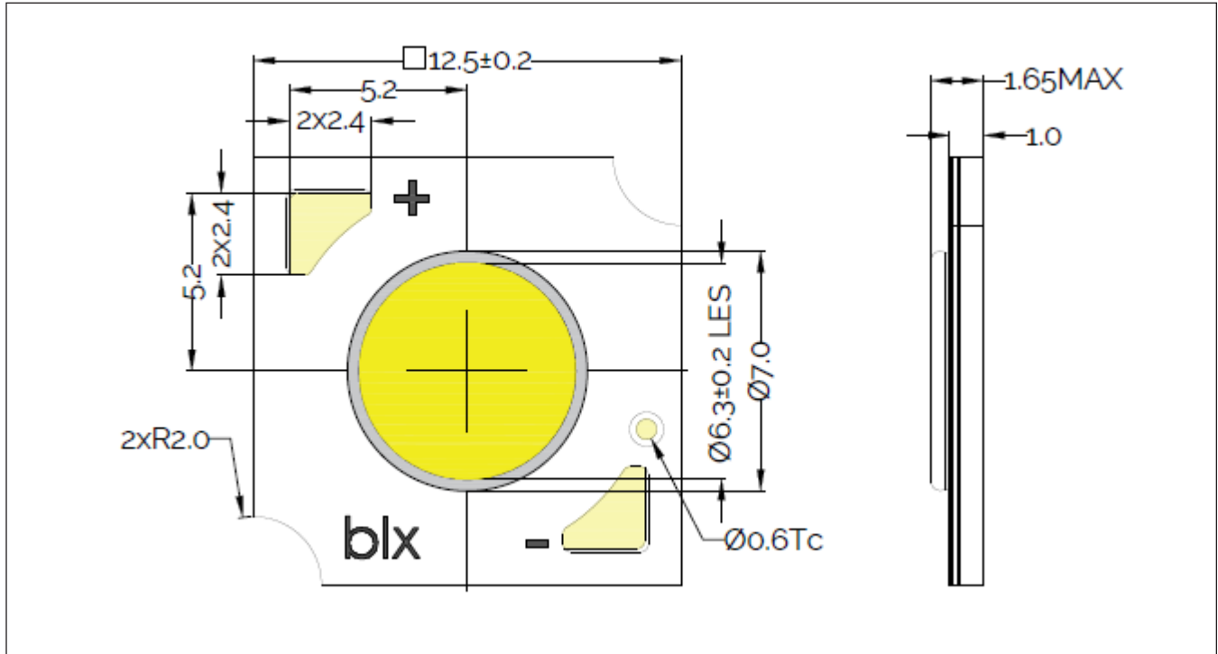
Figure 12: Drawing for V6 LED Array
