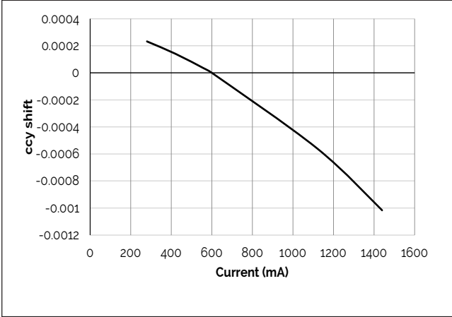
Figure 7: Drive Current vs. ccy Shift
