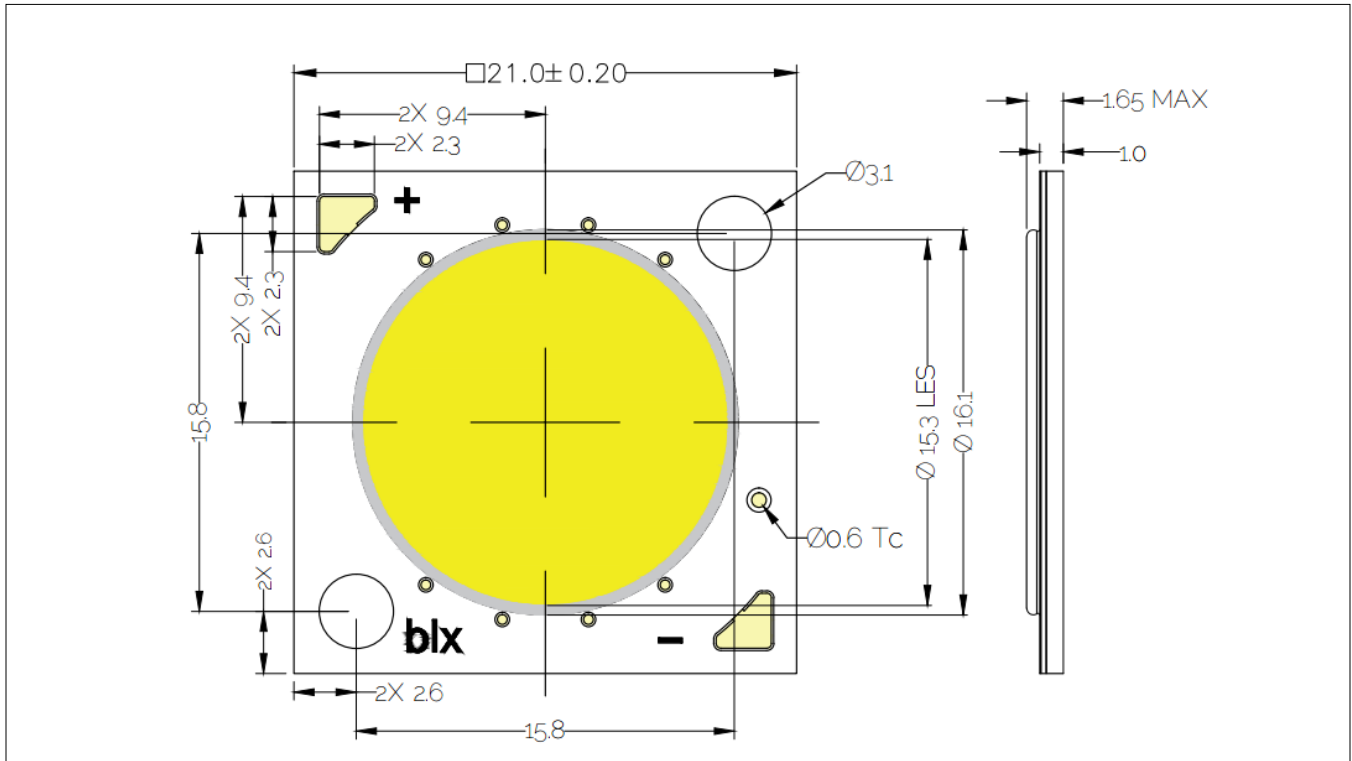
Figure 12: Drawing for V15 LED Array
