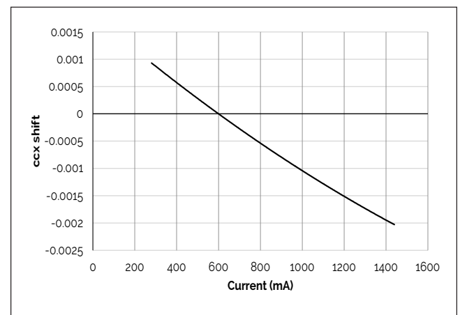
Figure 6: Drive Current vs. ccx Shift
