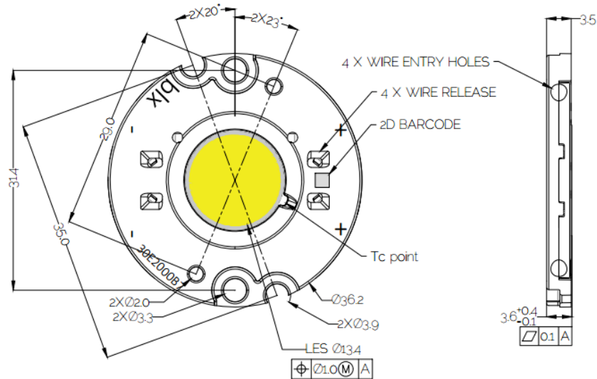
Figure 17: Drawing for Vero SE 13 LED Array
