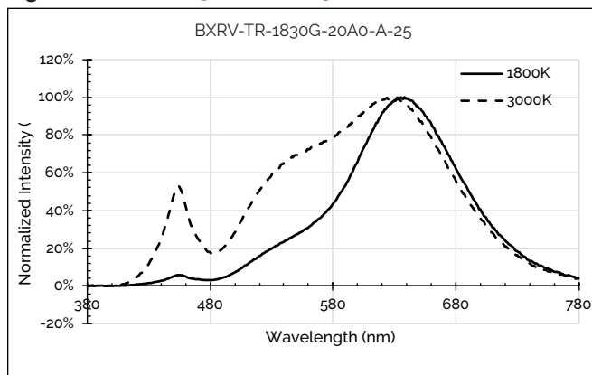
Figure 26: 1800K - 3000K with 90 CRI
